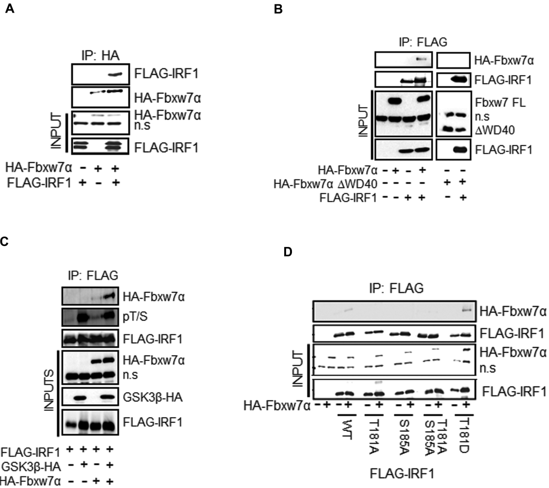
Figure 9. Fbxw7α interacts with phosphorylated IRF1 via T181. (A) Co-immunoprecipitation of HA-Fbxw7α in extracts of HEK293 cells, and western blots using anti-HA antibody to detect associated FLAG-IRF1. Cells were treated with MG132 for 6 h prior to lysis. Blots were re-probed with anti-HA to determine IP efficiency n.s. = non-specific band is indicated. (B) Co-IP experiment as in (A) but with anti-FLAG antibody to IP and western blot with anti-HA to detect complex formation with HA-Fbxw7α or a mutant lacking the WD40 domain (HA-Fbxw7α ΔWD40). (C) HA-Fbxw7α, GSK3β-HA and FLAG-IRF1 were co-expressed in HEK293 for 48 h, 6 h prior to lysis cells were treated with 10 μM MG132. Lysates were immunoprecipitated with anti-FLAG and probed with anti-HA to detect Fbxw7α interaction. The blots were also probed with the anti-pT/S antibody and FLAG to determine relative levels of IRF1 phosphorylation. (D) Immunoprecipitations as for (B) but with the inclusion of IRF1 T181A, S185A, T181A/S185A and T181D mutants.
