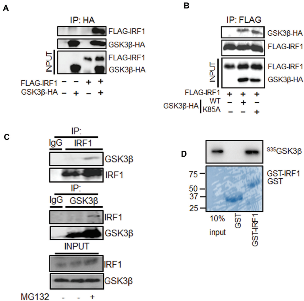
Figure 2. IRF1 interacts with GSK3β. (A) Extracts from HEK293 cells expressing FLAG-IRF1 and GSK3β-HA were immunoprecipitated with anti-HA. Shown are western blots used to reveal co-precipitated GSK3β-HA or FLAG-IRF1 proteins. Expression levels in the inputs (10%) are shown in the bottom panels. (B) As for (A), but using anti-FLAG immunoprecipitation and including kinase inactive GSK3β-HA (K85A) (C) Extracts from H3396 cells pre-treated with MG132 (10 μM) or DMSO for 3hr, immunoprecipitated with IgG, anti-IRF1 or anti-GSK3β antibodies to reveal endogenous complexes. (D) GST pull-down experiment using bacterially expressed, partially purified GST (27kda) or GST-IRF1 (63 KDa) immobilized on glutathione sepharose beads and incubated with in vitro transcribed/translated 35 [S]-methionine-labelled GSK3β-HA. Proteins retained on the beads were visualized by autoradiography. 10% input of radiolabeled product is shown as input. Lower panel shows a parallel CBB stained gel to show loading.
