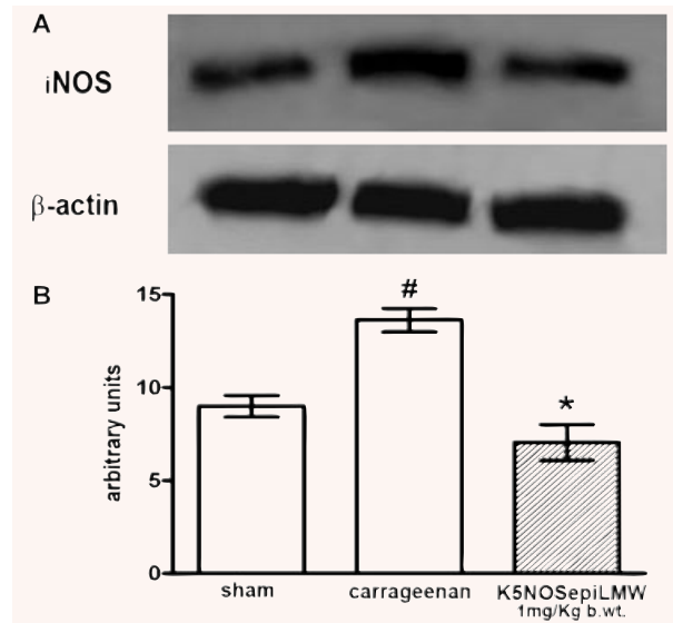
Fig. 2 iNOS protein expression evaluated by Western blot analysis in lung tissue samples from the different experimental groups, collected 4 hrs after carrageenan injection. Carrageenan increases iNOS expression, whereas pre-treatment with K5NOSeplLMW (1 mg/kg b.wt.) inhibits this effect (A). These data are confirmed by densitometric analysis (B). Significance of differences (one-way ANOVA, n = 8 ): # P < 0.001 versus sham-operated controls; * P < 0.001 versus carrageenan treated.
