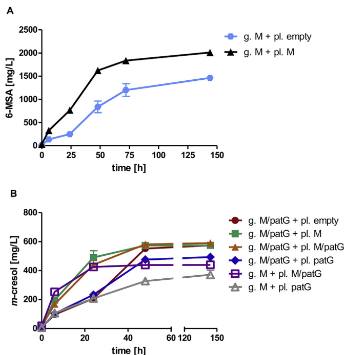
Fig. 8. Determination of the limiting factors for 6-MSA and m -cresol production. A) 6-MSA titers produced by strain JHY163 ( ura3::P^{popl}MSAS_{opt_{ngpA}} ) expressing additionally P^{popl}MSAS and opt_{ngpA} from multi-copy plasmid pJHV49 (pl. M; black) or as control the empty plasmid pRS42K (pl. Empty; light blue). B) m -cresol titers produced by strain JHY162 ( ura3::P^{popl}MSAS_{opt_{ngpA}_{opt_{patG}} ) carrying additionally as a control the empty plasmid pRS42K (pl. Empty; red), or expressing P^{popl}MSAS , opt_{ngpA} , opt_{patG} from pJHV53 (pl. M/patG; orange) or opt_{patG} from pJHV13 (pl. patG; blue) and strain JHY163 ( ura3::P^{popl}MSAS_{opt_{ngpA}} ) (g. M) expressing additionally P^{popl}MSAS , opt_{ngpA} , opt_{patG} from pJHV53 (pl. M/patG; purple) or opt_{patG} from pJHV13 (pl. patG; grey). High-OD fermentations (starting OD = 5) were performed in biological duplicates at 30 °C in YPD supplemented with G418 (error bars represent standard deviations). g. M. indicates genomic expression of MSAS/ngpA , g. M/patG indicates genomic expression of MSAS/ngpA and patG , + pl. indicates additional overexpression from multi-copy plasmids. (For interpretation of the references to color in this figure legend, the reader is referred to the Web version of this article.)
