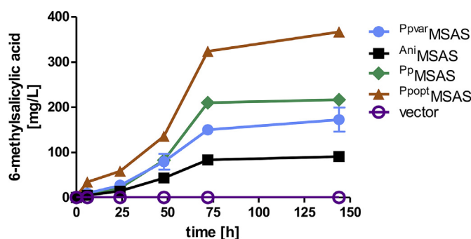
Fig. 3. 6-MSA production by different MSASs in high-OD fermentations. Yeast strain CEN.PK2-1C carrying the empty vectors pJHV7 and pRS62H as control (purple), and strains expressing ^{opt} npaA (pJHV2) and the MSAS variants ^{Ppvar} MSAS (pJHV17; light blue), ^{Ani} MSAS (pJHV5; black), ^{Pp} MSAS (pJHV11; green) or ^{Ppop} MSAS (pJHV36; orange) from multi-copy plasmids were inoculated at an OD of 9, and cultivated for 144 h at 30 °C in 25 mL YPD supplemented with G418 and hygromycin. 6-MSA concentrations were determined in the supernatants. Error bars represent the standard deviation of biological duplicates. (For interpretation of the references to color in this figure legend, the reader is referred to the Web version of this article.)
