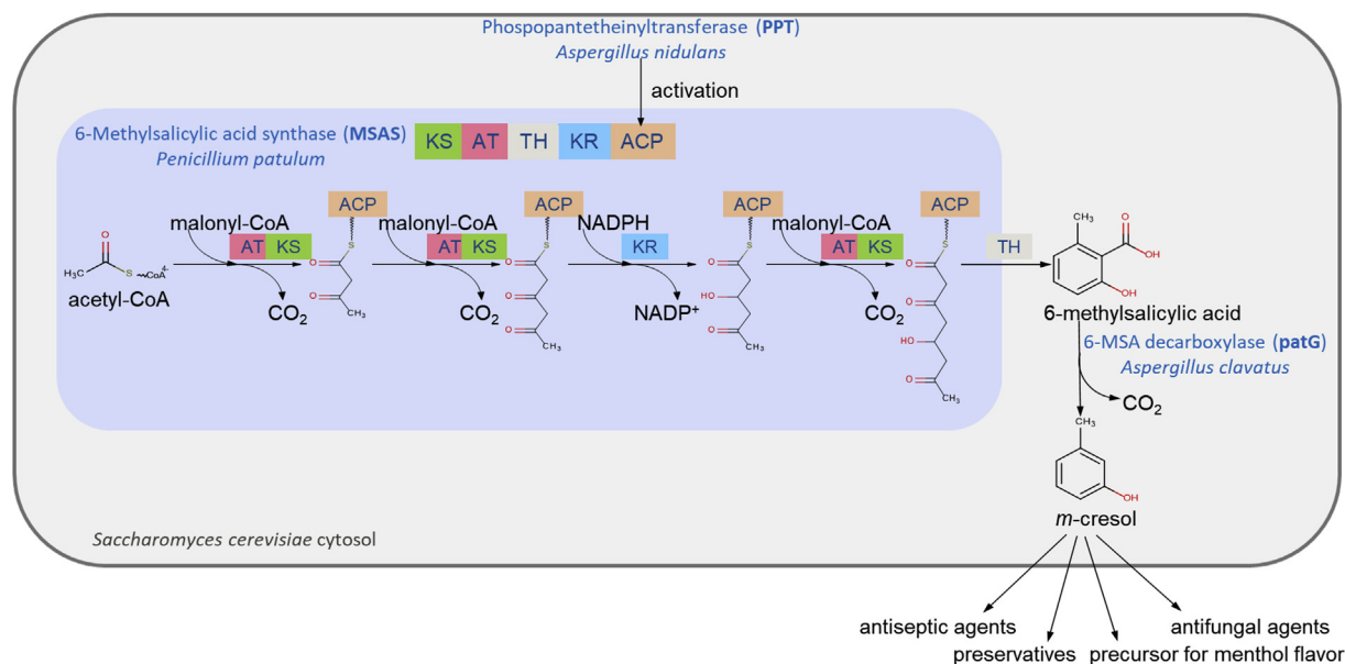
Fig. 1. Metabolic pathway for m -cresol production in S. cerevisiae via 6-methylsalicylic acid (6-MSA) synthesis. The 6-methylsalicylic acid synthase (MSAS) consists of multiple domains: the ketoacylsynthase (KS), acyltransferase (AT), thioester hydrolase (TH), ketoreductase (KR), and acyl carrier protein (ACP). MSAS must be activated by phosphopantetheinylation, and catalyzes the synthesis of 6-MSA from one acetyl-CoA and three malonyl-CoA under consumption of one NADPH. 6-MSA decarboxylase can further convert 6-MSA to m -cresol, valuable for the flavor and pharmaceutical industry. (For interpretation of the references to color in this figure legend, the reader is referred to the Web version of this article.)
