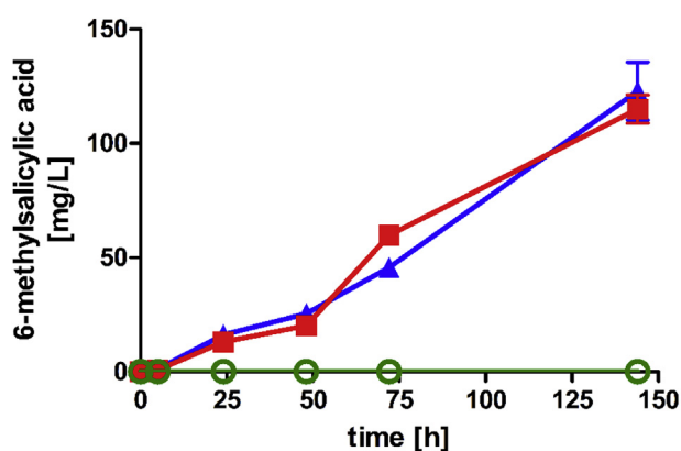
Fig. 2. 6-MSA formation with strain CEN.PK2-1C carrying the empty vectors pJHV7 and pRS62H as control (green circles), expressing ^{Ppvar} MSAS and native npaA from multi-copy plasmids pJHV17 and pJHV20 (red squares) and expressing ^{Ppvar} MSAS and codon-optimized ^{opt} npaA from multi-copy plasmids pJHV17 and pJHV2 (blue triangles). Cultures were inoculated at low OD (0.1) and cultivated for 144 h at 30 °C in 25 mL YPD supplemented with G418 and hygromycin. 6-MSA concentrations were determined in the supernatants. Error bars represent the standard deviation of biological duplicates. (For interpretation of the references to color in this figure legend, the reader is referred to the Web version of this article.)
