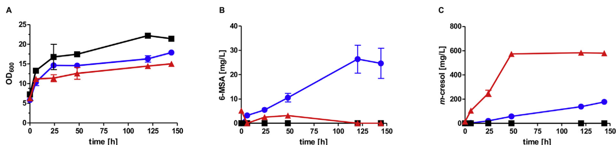
Fig. 7. Increase in m -cresol production by genomic integration of the pathway genes. Growth (A) and production of 6-MSA (B) and m -cresol (C) of CEN.PK2–1C expressing P^{popl}MSAS , opt_{ngpA} and opt_{patG} from multi-copy plasmid pJHV53 (blue) or from genome (strain JHY162; red). As control, the empty vector pRS42K was transformed into CEN.PK2–1C (black). High-OD fermentations (starting OD = 6) were performed in biological duplicates at 30 °C in YPD supplemented with G418 for plasmid maintenance (error bars represent standard deviations). (For interpretation of the references to color in this figure legend, the reader is referred to the Web version of this article.)
