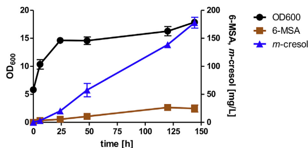
Fig. 6. Production of the intermediate 6-MSA (orange), final product m -cresol (blue) and growth (black) of CEN.PK2-1C expressing Ppopt MSAS , opt mpgA and opt patG from multi-copy plasmid pJHV53. Fermentations (starting OD = 5) were performed in biological duplicates at 30 °C in YPD supplemented with G418. 6-MSA and m -cresol concentrations were determined in the supernatants. Error bars represent standard deviation of biological duplicates. (For interpretation of the references to color in this figure legend, the reader is referred to the Web version of this article.)
