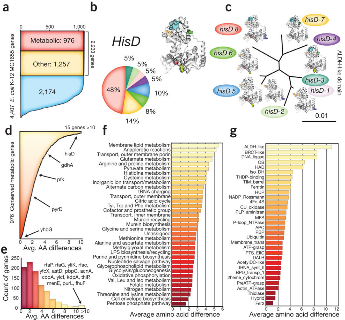
Figure 4. Comparison of ML1515 to sequence variations in 1,122 clinical Isolates of E. coli . (a) Counts for each E. coli K-12 MG1655 gene in 1,122 sequenced strains of E. coli are shown. (b) Histidine pathways showed high levels of amino acid differences among genes involved. The pie chart represents the percentage of strains that contain unique hisD alleles. The hisD 116 allele of E. coli K-12 MG1655 is present in only 19 (1.7%) of the sequenced strains. (c) Structural biology methods can reveal the effect of mutations. (d) 976 genes with metabolic functions are conserved across 99% of E. coli strains and this core set also has mutations. The bar chart shows the average number of amino acid mutations in these core genes for 1,122 strains of E. coli . (e) A histogram showing how many genes have a certain number of average mutations. (f) Amino acid mutations are compared for major metabolic
