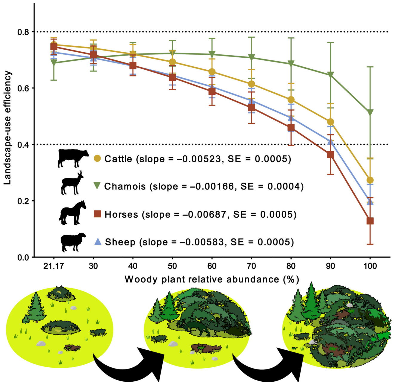
Figure 3. Evolution of the landscape-use efficiencies (LUE) of Pyrenean chamois and seasonal livestock along different scenarios of woody plant expansion. Slopes of the linear regression are also reported for each species
