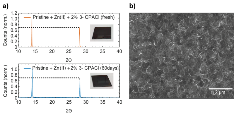
Figure 4. (a) XRD patterns of freshly made and aged perovskite containing Zn(II) and 3-CPACI. Inset: picture films before and after aging. (b) Low-magnification (20 000x) SEM image of perovskite containing Zn(II) and 3-CPACI showing a homogeneous, dense, and pinhole-free layer.
