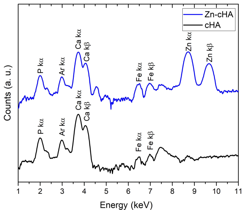
Figure S2 SR- \mu XRF spectra of cHA and Zn-cHA microspheres (region I).
