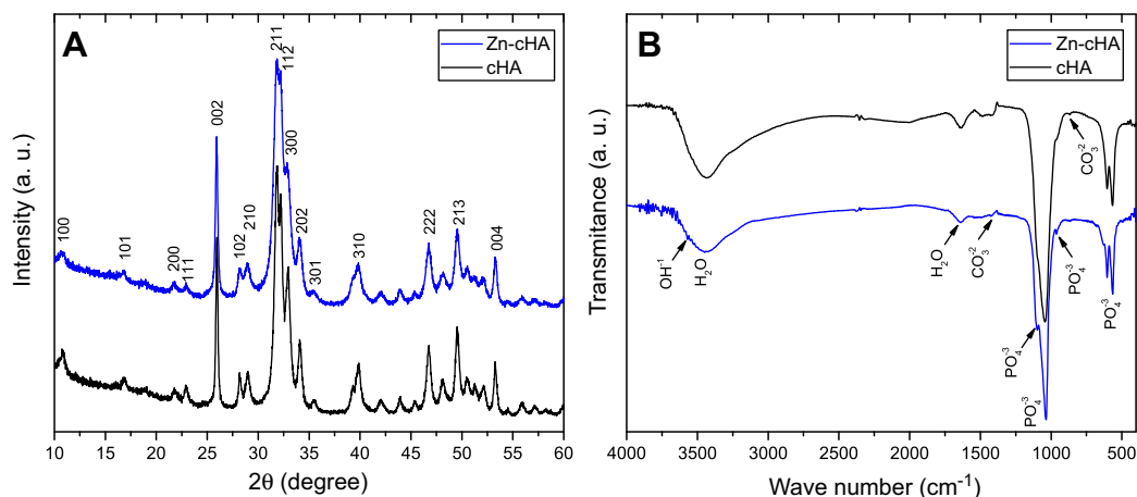
Figure 1 XRD patterns (A) and FTIR spectra (B) of Zn-cHA and cHA powders.
