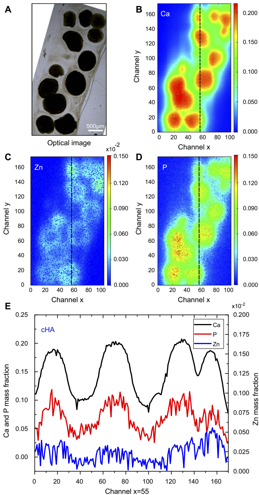
Figure 9 cHA microspheres implanted for 6 months in rat calvaria (region I). (A) Optical image and (B–D) Ca, Zn and P SR-μXRF elemental mapping; (E) Mass fraction profile of Ca, P and Zn along channel 55 (dash lines).
