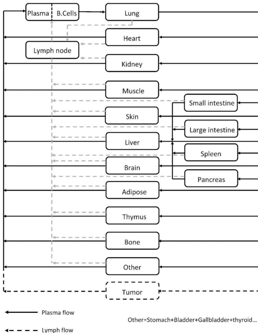
Figure-1: Structure of the whole-body platform PBPK model. All organs are represented by a rectangular compartment, and connected in an anatomical manner with blood flow (solid arrows) and lymphatic flow (dashed arrows). Arrows represent the direction of the flow. Each tissue within this model, except blood and lymph node, is divided into sub-compartments, as shown in Figure-2.
