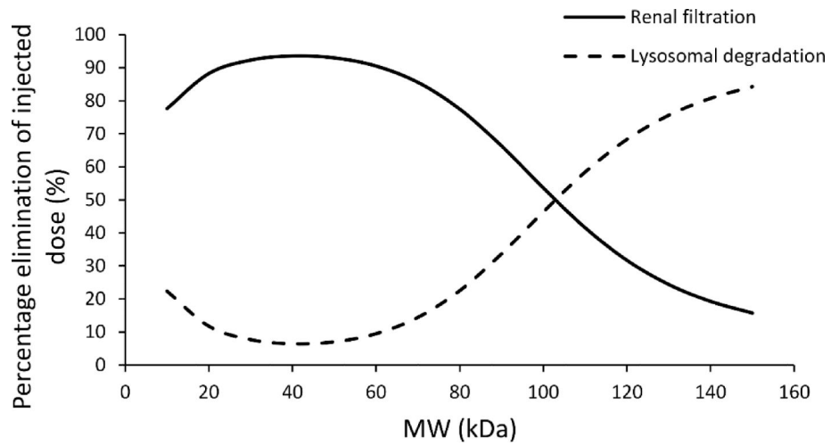
Figure-7: Model simulated relationship for relative (percentage) contribution of renal filtration and lysosomal degradation pathways towards the elimination of different size proteins. Solid line represents renal filtration and dashed line represents lysosomal degradation.
