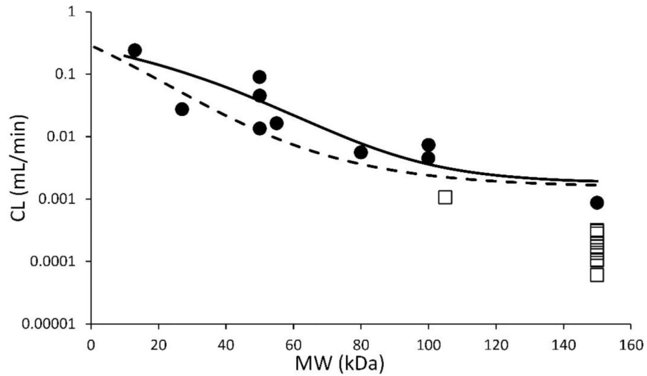
Figure-6: Model simulated clearance (CL) vs. molecular weight relationship. Solid line represents the clearance values simulated using the PBPB model. Dashed line represents our previous reported CL vs. MW relationship based on compartmental modeling [11]. Each closed circle represents NCA calculated CL value for a given protein. Open squares represents NCA calculated CL values for scFv-Fc or IgG in normal mice.
