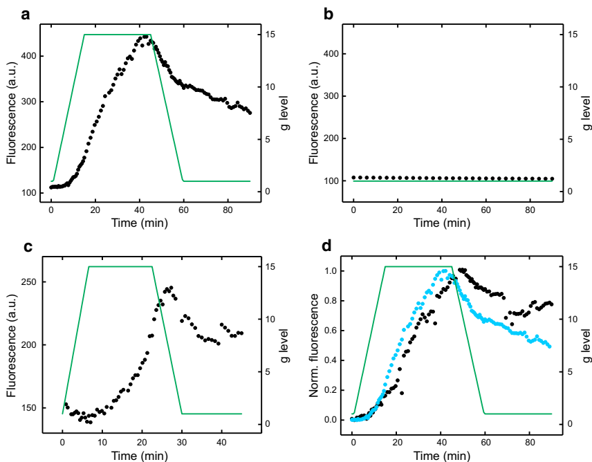
FIGURE 3 (a) Fluorescence response of 2 in MC3T3-E1 cells ( black ) as g level ( green ) is changed, with a 15-min ramp. (b) Control MC3T3-E1 cells showing no change in 2 fluorescence ( black ) as g level ( green ) is held at 1 \times g are shown. (c) The fluorescence response of 2 in MC3T3-E1 cells ( black ) as g level ( green ) is changed with a 7.5-min ramp is shown. (d) A normalized fluorescence response of cells treated by previous hypergravity exposure and relaxation, before a second hypergravity exposure ( black ), compared with cells with no previous hypergravity exposure ( blue ) is shown. To see this figure in color, go online.
