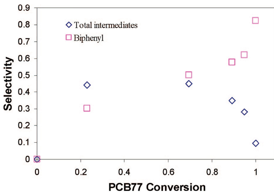
Figure 9. Selectivity for biphenyl and the intermediates as a function of PCB 77 conversion.
