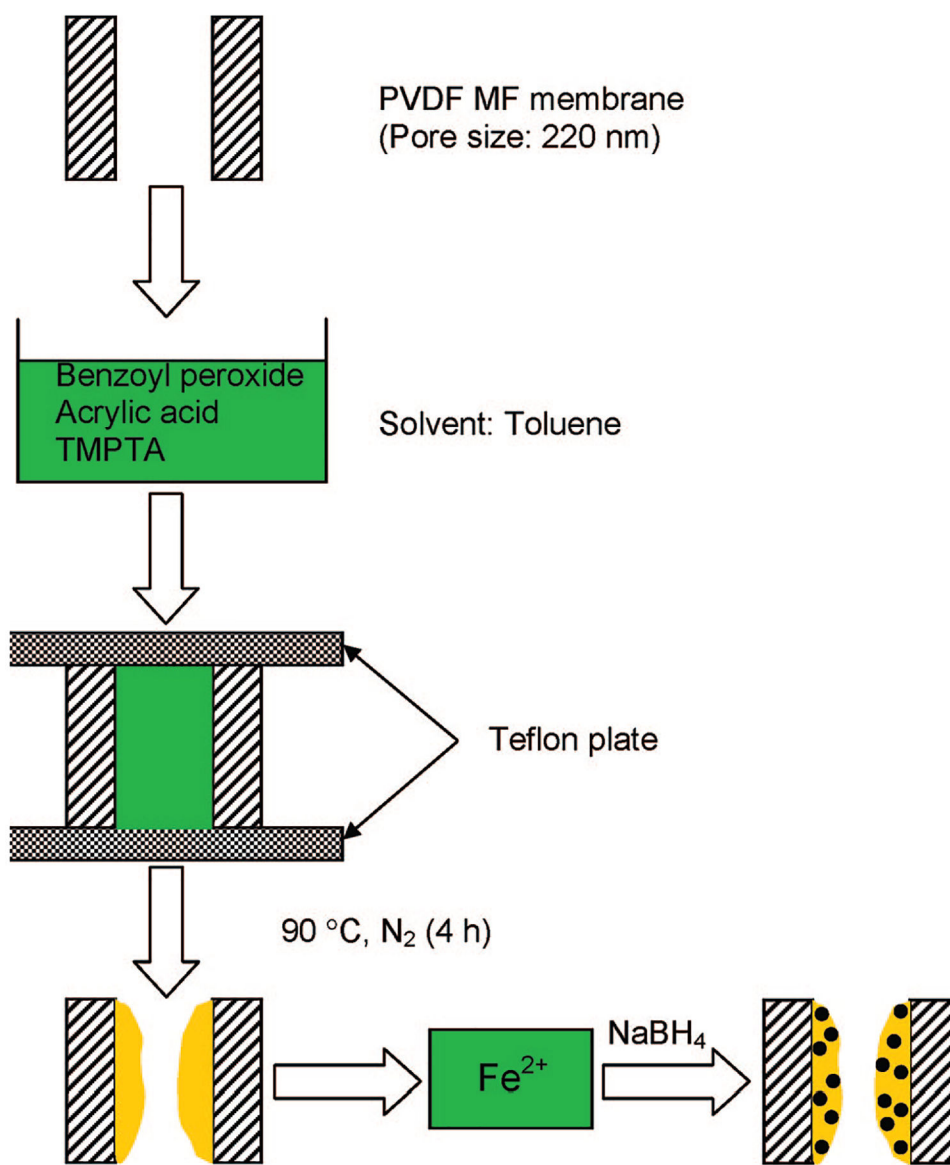
Figure 1. Preparation Fe 0 nanoparticles in PAA functionalized PVDF MF membranes by in situ polymerization of acrylic acid.
