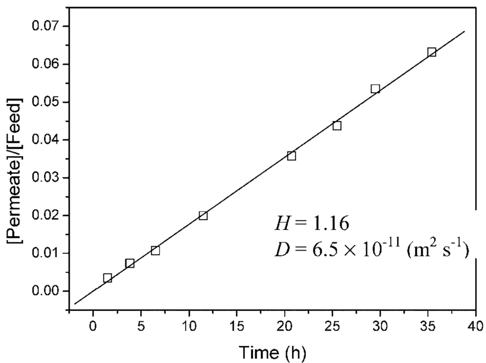
Figure 6. Experimental values of DiCB diffusion through the PAA/PVDF membrane containing deactivated Fe nanoparticles. Membrane thickness: 125 \times 10^{-6} m. Membrane area: 3.5 \text{ cm}^2 .
