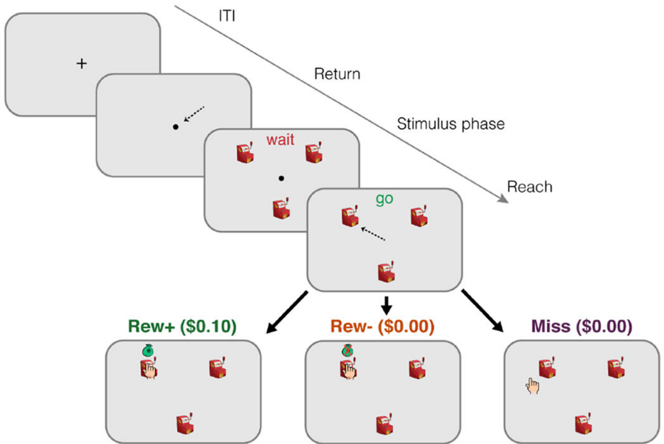
Figure 1: Task Design.
