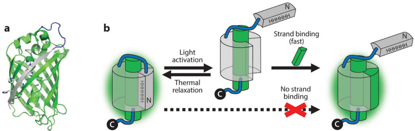
Figure 7. (a) Structure (PDB ID: 6B7R) (25) and (b) light activation of the strand-11 truncated protein. The N-terminal His tag (shown in gray ) binds as a new \beta -strand to the vacant spot left by removal of the native 11th strand. Light irradiation displaces the bound His tag and allows for binding of added synthetic peptides (shown in green ). Figure adapted with permission from Reference 25.
