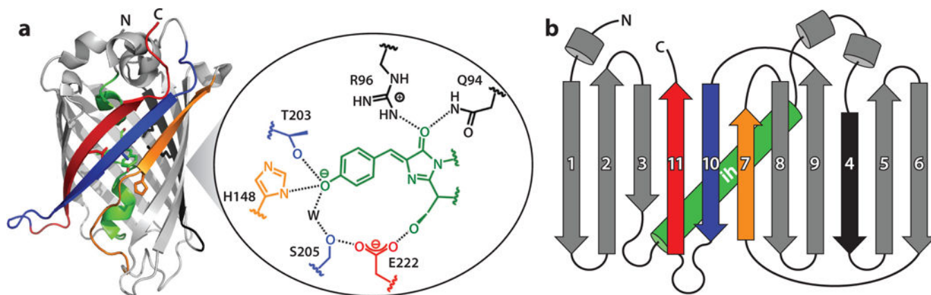
Figure 2. Green fluorescent protein (GFP) structure and topology. (a) Ribbon structure of GFP (PDB ID: 2B3P) (103) highlighting the chromophore environment and the proximity of the N- and C-termini. The internal \alpha -helix that contains the chromophore is shown in green, while \beta -strands 4, 7, 10, and 11 are shown in black, orange, blue, and red, respectively. (b) Topology of GFP's 11 \beta -strands and internal \alpha -helix (ih). Figure adapted with permission from Reference 78.
