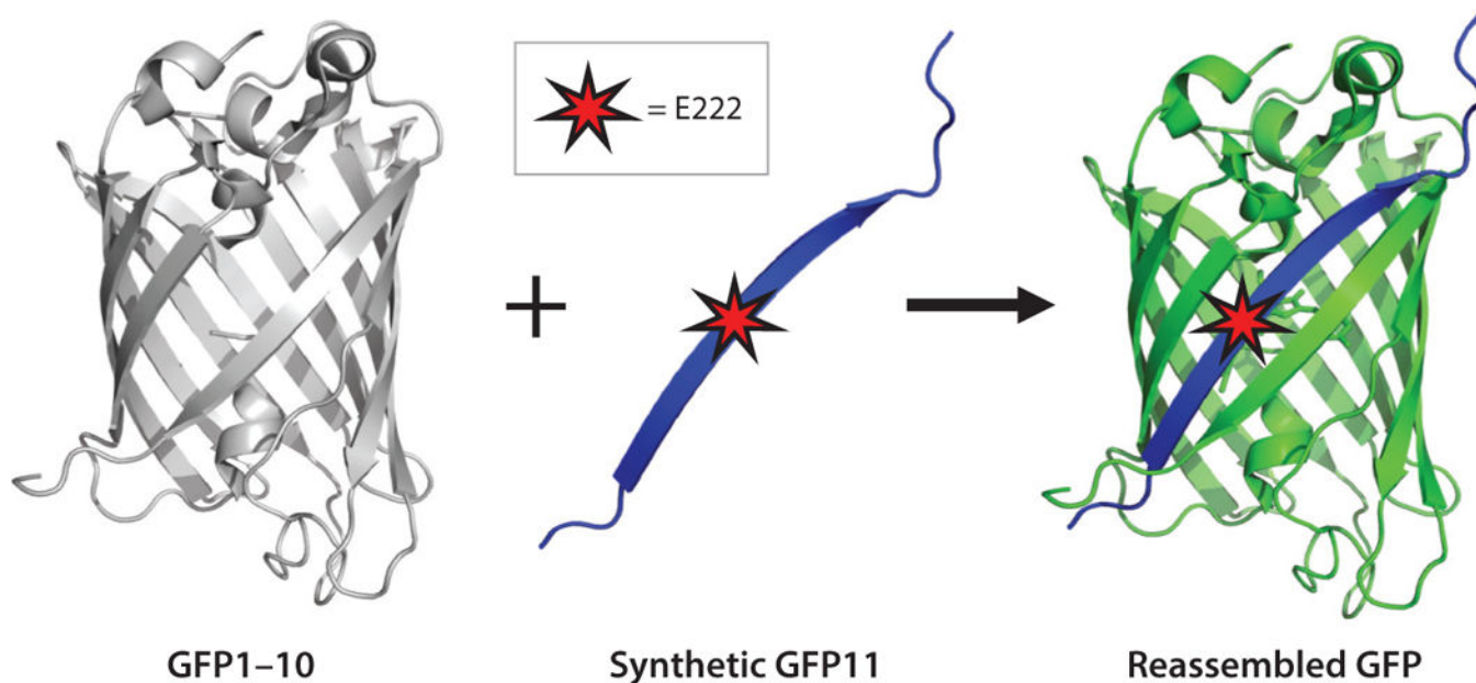
Figure 4. Schematic diagram illustrating split protein reassembly between recombinant GFP1-10 and a synthetic GFP11 peptide with subsequent chromophore maturation (PDB ID: 2B3P) (103). Mutations at E222 tune the photophysical properties of the chromophore. Note that the 3D structure of the truncated protein shown in gray is not currently known. Figure adapted with permission from Reference 59.
