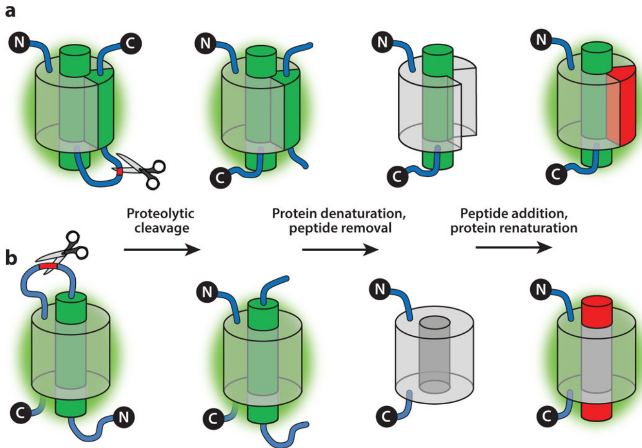
Figure 5. Schematic illustrating the required experimental steps for the synthetic control of green fluorescent protein, applied to either (a) the strand 7, 10, or 11 system or (b) the internal \alpha -helix system. The loop between the terminal secondary structural element and the rest of the protein is proteolytically cleaved. The noncovalently bound complex is denatured, and the fragments are separated with size exclusion chromatography. Refolding of the larger fragment, referred to as the denatured truncated protein (shown in gray as if folded), with synthetic peptide (shown in red ) corresponding to the missing structural element yields a fluorescent species resembling the native protein. Point mutations on the synthetic peptides that cause color shifts and/or protonation state changes can be introduced in this manner. Figure adapted with permission from Reference 60.
