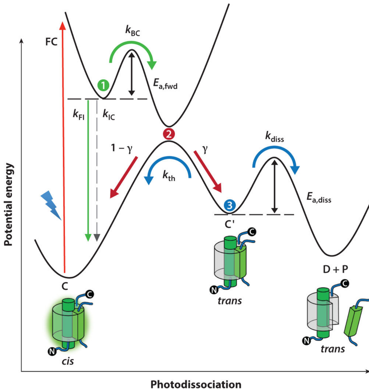
Figure 9. Potential energy curves for photodissociation, highlighting relevant parameters. Branching points are shown as circled numbers and are color coded to match their associated processes: 1 represents the excited-state barrier partitioning fluorescence and isomerization; 2 represents the photochemical funnel, which divides aborted from successful isomerization; and 3 represents branching of strand dissociation and thermal relaxation. Abbreviations: C, noncovalently bound fluorescent protein complex with a cis chromophore in the ground electronic state; C', noncovalently bound fluorescent protein complex with a trans
