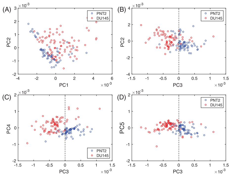
FIGURE 5 PCA scores plots. (A) Scores generated by PC1 and PC2. (B) Scores generated by PC3 and PC2. (C) Scores generated by PC3 and PC4. (D) Scores generated by PC3 and PC5
