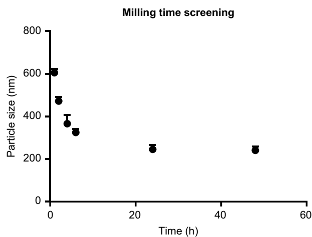
Figure S1 Dependence of particle size (nm) on the milling time (hrs) (n=3), particle size decreased as milling time increase up to 24 hrs.
