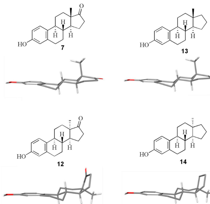
Figure 1. The structure of 13\alpha -epimeric estrones ( 7 and 12 ) and their 17-deoxy counterparts ( 13 and 14 ).
