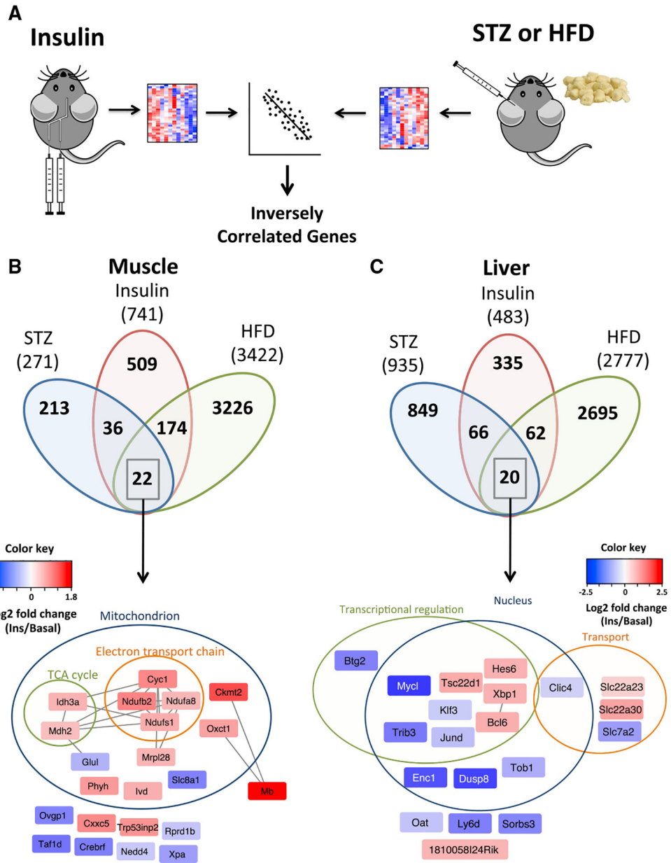
Figure 5. Genes Inversely Regulated during the Euglycemic Insulin Clamp, STZ Diabetes, and HFD Obesity in Muscle and Liver (A) Schematics of insulin clamp and STZ or HFD dataset comparisons. (B and C) Overlap of inversely correlated genes among insulin, STZ diabetes, and HFD obesity in muscle (B) and liver (C). Genes representing the overlap of all conditions grouped by functional annotation and cellular localization are indicated. Edges represent predicted protein-protein interactions from STRING. Colors of nodes are log 2 fold change values of regulation by insulin. See also Table S4.
