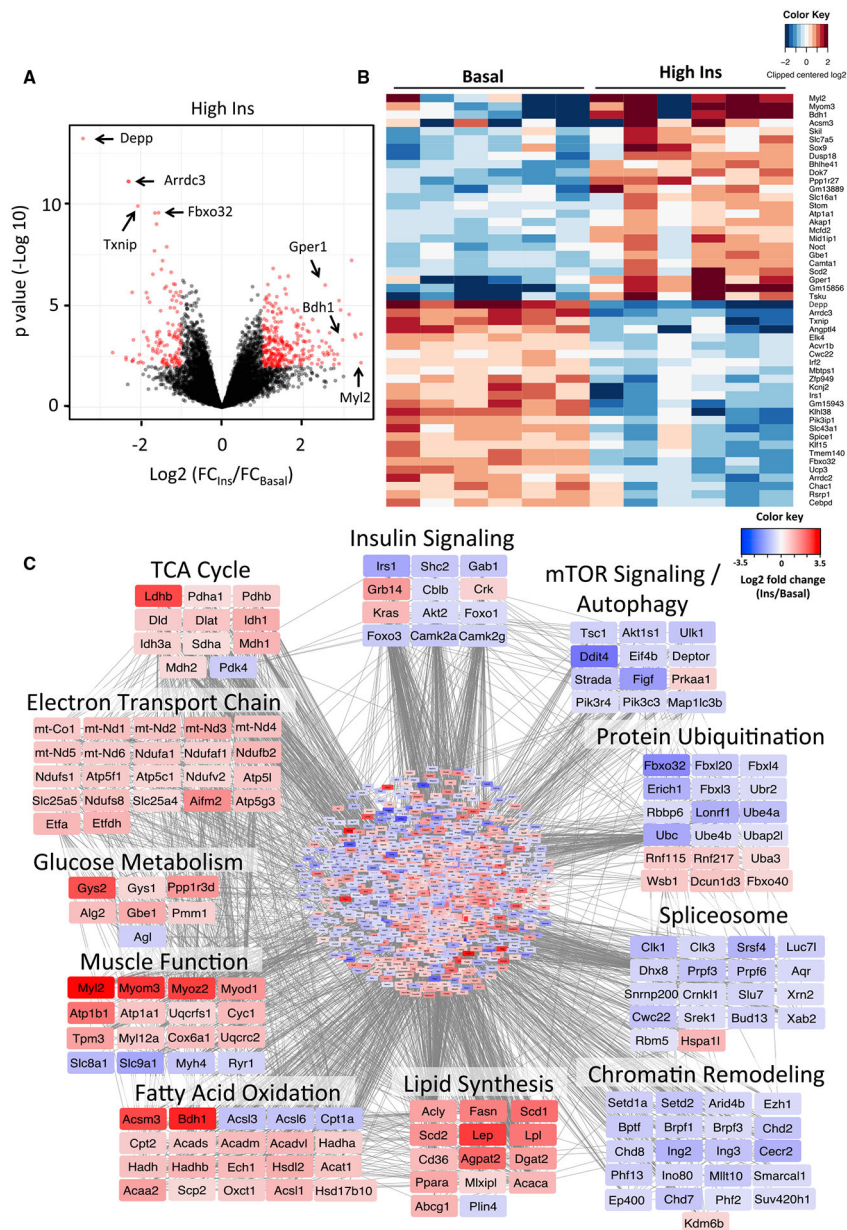
Figure 2. Insulin Regulation of Gene Expression in Skeletal Muscle (A) Volcano plot showing distribution of differentially expressed genes (in red) by high insulin at 3 h compared to basal on the log 2 scale. (B) Heatmap showing the top 50 insulin-regulated genes. See also Figure S2. (C) Network of predicted protein-protein interactions from STRING analysis (Szklarczyk et al., 2017) using insulin-regulated genes in muscle as input. 1,406 nodes and 6,369 interactions were detected ( p < 1 \times 10^{-16} ). Colors of nodes represent log 2 fold change values of insulin regulation. See also Figure S3 and Tables S2 and S3.
