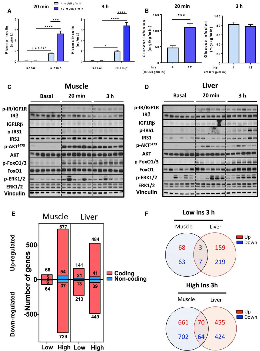
Figure 1. Euglycemic Clamp, Insulin Signaling, and Gene Expression in Muscle and Liver (A) Plasma insulin levels before and after hyperinsulinemic-euglycemic clamp with 4 or 12 mU/kg/min insulin infusion for 20 min or 3 h (n = 2–4). Data are mean ± SEM (n = 6), *p < 0.05, ***p < 0.01, ****p < 0.0001, two-way ANOVA. (B) Glucose infusion rates indicated as average of t = 10–15 min for the 20 min clamp and t = 120–150 min for the 3 h clamp. ***p < 0.001, Student’s t test. Data are mean ± SEM. (C and D) Insulin signaling in (C) muscle and (D) liver from mice infused with high insulin for 20 min or 3 h (n = 6). For basal levels, 3 samples from saline-infused mice at each time point were used. See also Figure S1. (E) Number of regulated genes by low- and high-dose insulin at 3 h (FDR < 0.1). (F) Venn diagrams showing the overlap of up- and down-regulated genes in muscle and liver under low and high insulin conditions at 3 h.
