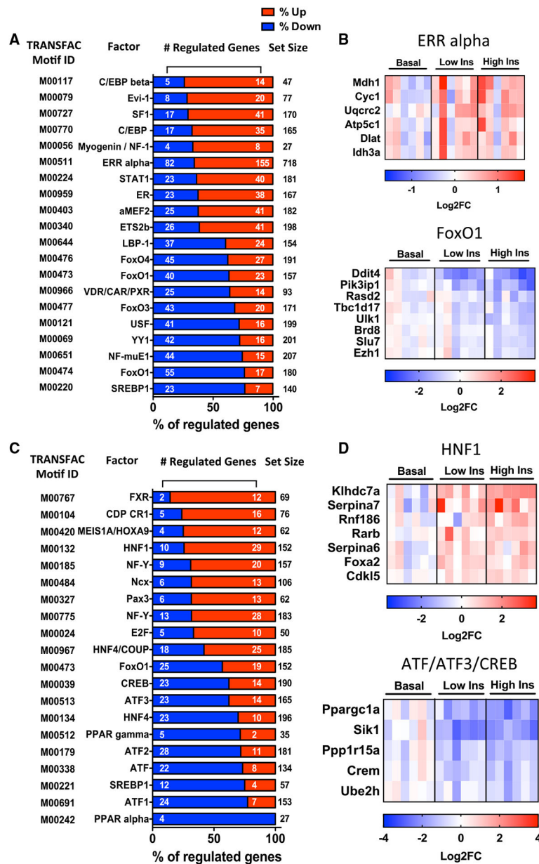
Figure 4. Transcription Factor Motifs Enriched in Insulin-Regulated Genes in Muscle and Liver (A and C) Overrepresented transcription factor motifs within 2 kb of TSS in (A) muscle and (C) liver. Plots are percentages of predicted target genes that are significantly up- or downregulated by insulin (FDR < 0.1). Enrichment analysis was performed using data from low and high insulin samples combined (n = 12). (B) Examples of genes in muscle showing enrichment for ERR \alpha (top) and FOXO1 (bottom) binding motifs. (D) Examples of genes in liver showing enrichment for HNF1 (top) and ATF protein (BATF, ATF3, and CREB) (bottom) binding motifs. See also Figure S4.
