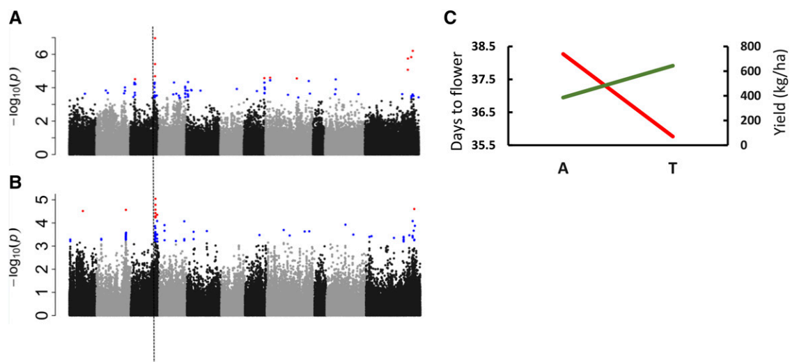
Figure 3 MLM GWAS analysis for BASE panels. A. Yield GWAS results for the panel grown under heat in Honduras and Puerto Rico in 2016. B. Days to flower GWAS results for the panel grown under heat in Honduras and Puerto Rico in 2016. The P value cutoff for the two GWAS, as determined using the Bonferroni test based on the effective number of SNPs was -\log_{10}(P) = 4.10 . C. Allelic performance for SNP S03_40504942 for days to flower (red) and yield (green) grown under heat in Honduras and Puerto Rico in 2016.
