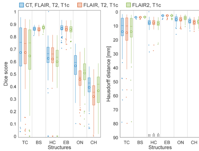
Figure 5: Boxplots of Dice scores (left) and Hausdorff distances (right) for structures in the Copenhagen dataset, for three data combinations in blue, red and green, respectively. 70 subjects in total. On each box, the central line is the median, the circle is the mean and the edges of the box are the 25th and 75th percentiles. Outliers are shown as dots. Black dots at the bottom of the Hausdorff distance boxplot indicate structures for which scores could not be calculated due to missing ground truth. Note that scores for the left and right structures are included separately in the box plots for HC, EB and ON.
