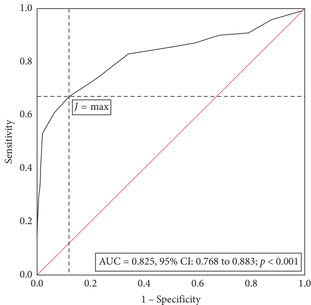
FIGURE 1: Summary receiver operating characteristic (ROC) curve for BMI as an anthropometric marker to distinguish benign from malignant breast tumors. The red line shows an equal proportion of correctly classified breast cancer sample and incorrectly classifies samples without breast cancer (random classification). The J max ( \max(Se + Sp - 1) ) corresponds to a Se = 0.67 and a Sp = 0.88 for a cutoff > 29.5 \text{ kg/m}^2 (BMI) for the breast cancer sample.
