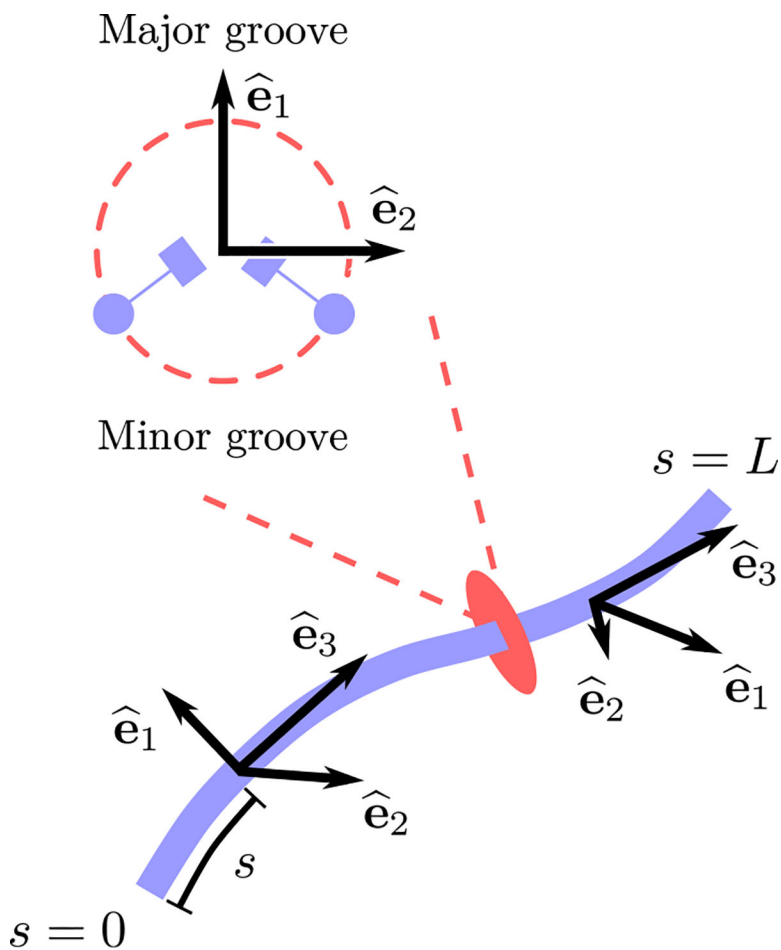
FIG. 1. Bottom: The configuration of a twistable elastic rod can be mathematically described with an orthonormal set of vectors \{\hat{e}_1, \hat{e}_2, \hat{e}_3\} assigned to every point s along the rod. The vector \hat{e}_3 is the tangent to the curve, and describes the bending fluctuations along the rod. Top: Cross-section of the rod, indicating how the remaining vectors \hat{e}_1 and \hat{e}_2 which describe the torsional state, may be chosen in the particular case of DNA.
