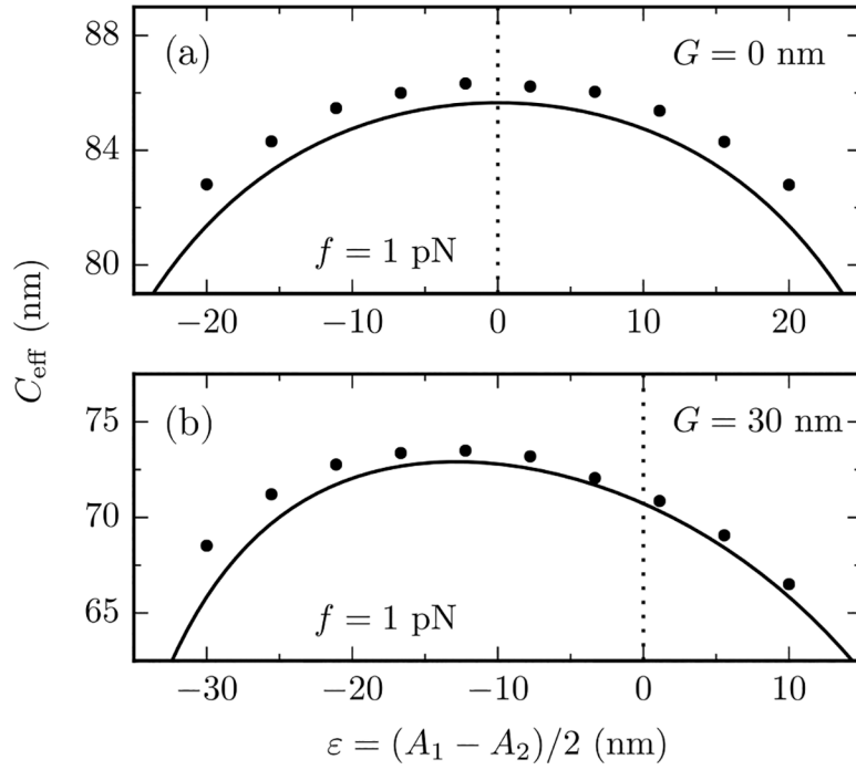
FIG. 4. Effect of bending anisotropy ( A_1 - A_2 ) on the effector stiffness at a fixed force f = 1 pN with (a) G = 0 and (b) G = 30 nm. Numerical data from Monte Carlo simulations of the triad model (points) are in good agreement with the analytical, nonperturbative predictions of Eq. (28) (solid lines). The vertical dashed lines indicate the isotropic case ( \epsilon = 0 ). A nonvanishing twist-bend coupling (lower panel) induces a \epsilon \rightarrow -\epsilon symmetry breaking. Error of Monte Carlo data are smaller than symbol sizes.
