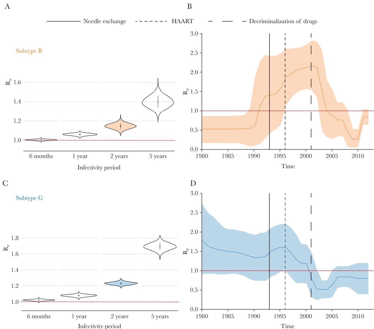
Figure 3. A and C, Effective reproductive number ( R_e ) estimates obtained using the constant rate birth-death model (ie, model 1; constant R_e ) under different assumptions of infectious period (6 months–5 years; rate of becoming uninfected, 2.0–0.2) for subtypes B (A) and G (C). The vertical lines in the middle of the violin plots represent the interquartile range. The filled with color violin plots (A) represent the value of R_e assuming the infectious period of 2 years. The horizontal red dotted line represents the epidemiological threshold ( R_e = 1 ). B and D, R_e estimates obtained using the birth-death skyline model (ie, model 2) over 10 equidistant intervals between the tree height and the most recent tip in the analysis for subtype B (B) and G (D), assuming an infectious period of 2 years. The shaded area represents the 95% Bayesian credible interval. The horizontal red dotted line represents the epidemiological threshold ( R_e = 1 ). Vertical lines correspond to the time of introduction of major interventions to prevent human immunodeficiency virus infection. HAART, highly active antiretroviral therapy.
