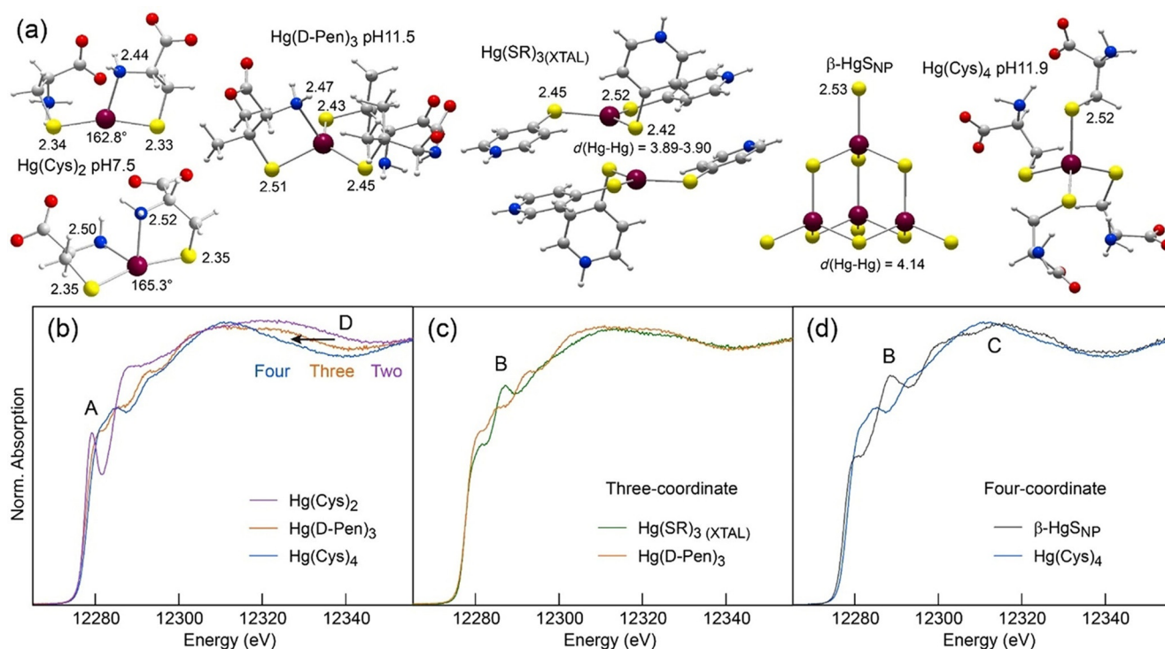
Figure 4. Sensitivity of L_3 -edge HR-XANES to the bonding environment of Hg. (a) Structure of the Hg complexes. (b–d) Spectra of two-, three-, and four-coordinate Hg-thiolate and Hg-sulfide references. The \text{Hg}(\text{Cys})_2 complex was prepared at a Cys:Hg molar ratio of 2 and pH 7.5, the \text{Hg}(\text{D-Pen})_3 complex at D-Pen:Hg = 10.0 and pH 11.5, and \text{Hg}(\text{Cys})_4 at Cys:Hg = 10.0 and pH 11.9. Their structure was optimized geometrically (MP2-RI/def2-TZVP-ecp [67] ), and the \text{Hg}(\text{SR})_3 complex and \beta\text{-HgS}_{\text{NP}} model are X-ray crystal structures. Peak B is diagnostic of Hg–Hg pairs. Bond lengths are in angstroms. Dark red, Hg; yellow, S; blue, N; red, O; gray, C; light gray, H.
