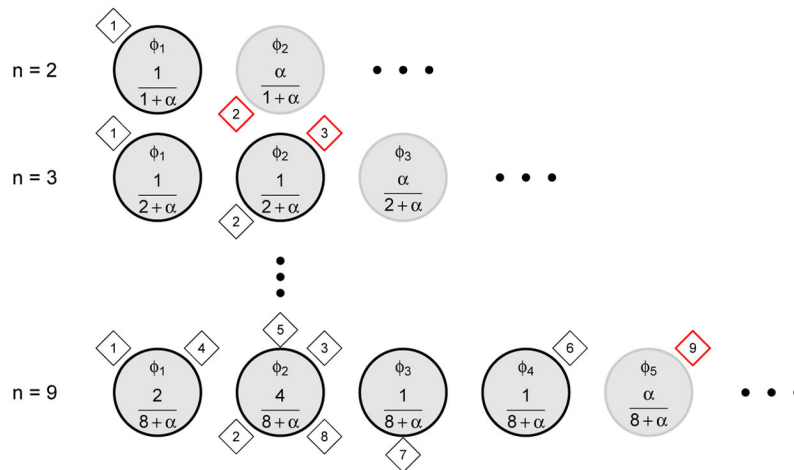
Figure 3: An illustration of the Chinese Restaurant Process. In the CRP metaphor, imagine a Chinese restaurant with an infinite number of tables. Customers (individual data entries, shown as diamonds) enter into the restaurant one by one and are seated at tables (discrete clusters, shown as circles), in the order in which they enter into the restaurant. There are parameters associated with the clusters, represented as \varphi_k = [\mu_k, \tau_k] for the cluster means and precisions. The first customer who enters into the restaurant always sits at the first table. The second customer enters and sits at the first table with probability 1/(1 + \alpha) , and the second table with probability \alpha/(1+\alpha) , where \alpha is a positive real number (top row, where i = 2 ). When the third customer enters the restaurant, he or she sits at each of the occupied table with a probability proportional to the number of previous customers already sitting there, and at the next unoccupied table with probability proportional to \alpha .
