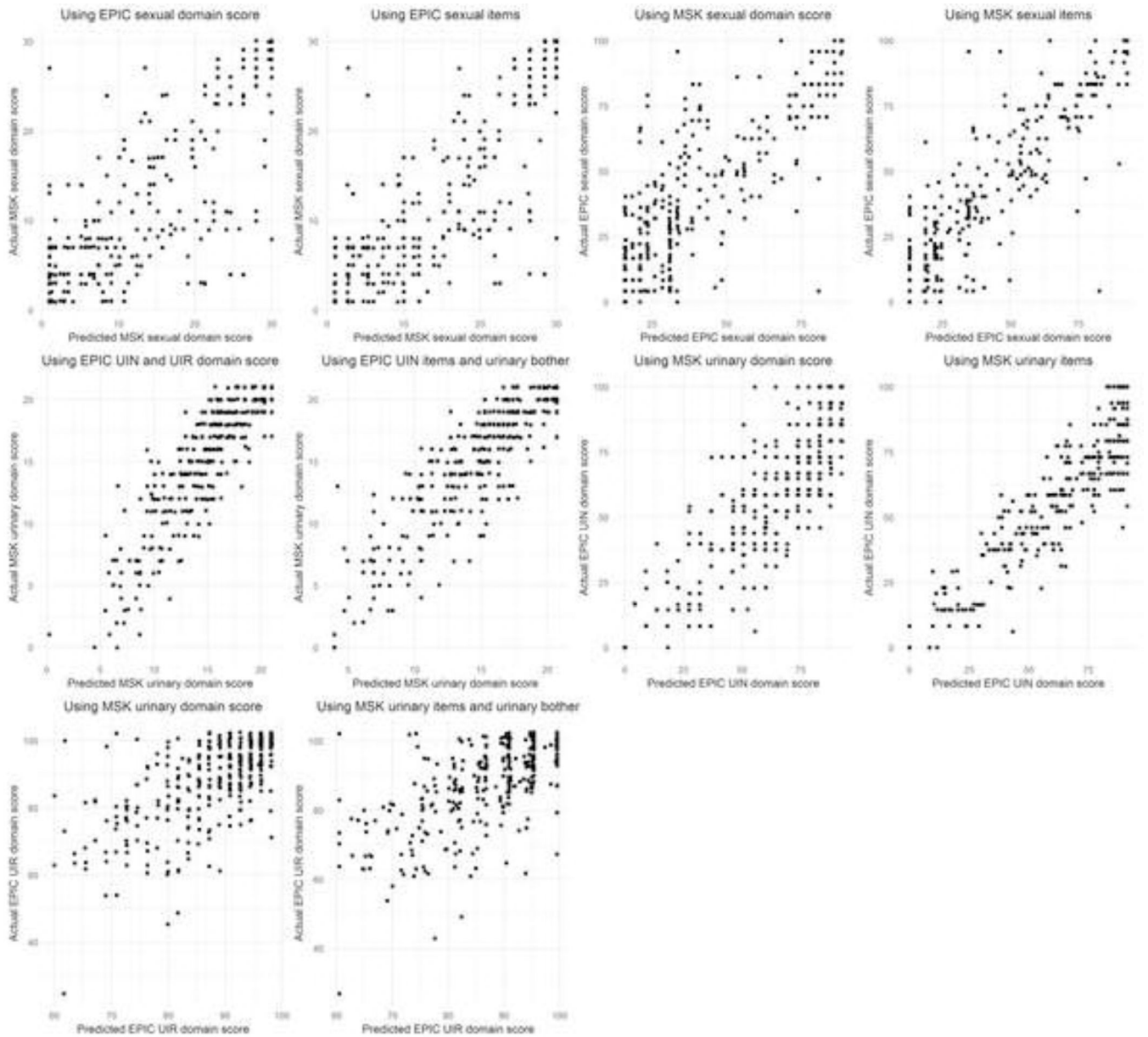
Fig. 2. Scatter plots comparing predicted versus actual domain scores to assess model calibration in the post-radical prostatectomy test set. It should be noted that the points have been slightly shifted randomly to minimize overlap.
