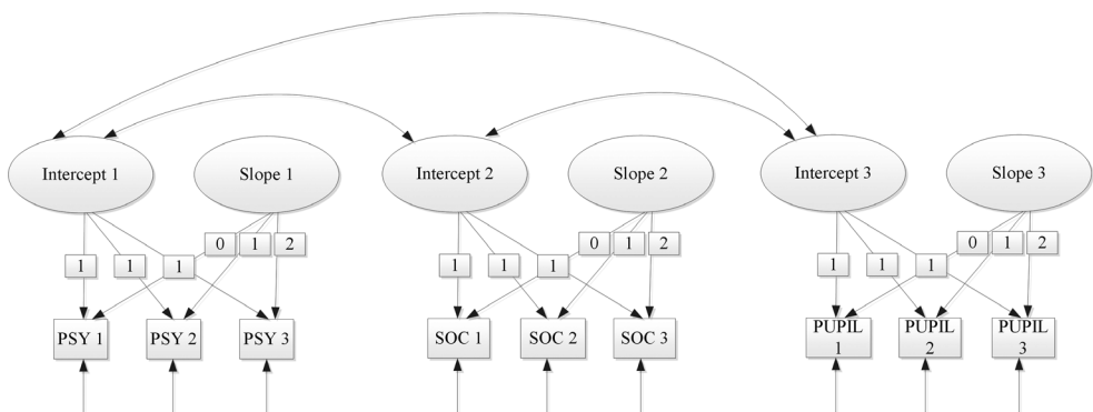
Figure 3. Multivariate latent growth curve model depicting the growth of stress causes.
