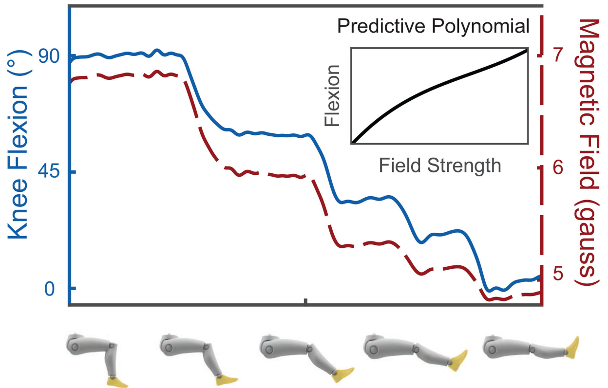
Figure 1: Sensor calibration was performed by placing the knee in 5 arbitrary positions between 0 and 90 degrees and fitting a 3 rd order polynomial (inset) to the magnetometer-accelerometer data.
