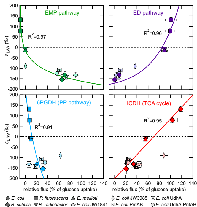
Fig. 2. Correlations between lipid/water fractionation ( \epsilon_{\text{L}/\text{W}} ) and the relative carbon flux through 6PGDH and ICDH as well as the EMP and ED pathways. Relationships were derived from E. coli , B. subtilis , P. fluorescens strains WCS368 and 2-79, R. radiobacter , and E. meliloti . In addition, five E. coli knockout mutants lacking specific dehydrogenase and transhydrogenase genes (text) are shown in light colors. Plotted \epsilon_{\text{L}/\text{W}} values are calculated between the culture medium and abundance-weighted mean \delta^2\text{H} values of fatty acids. The error bars represent the corresponding abundance-weighted SD. Note that some error bars are smaller than marker sizes.
