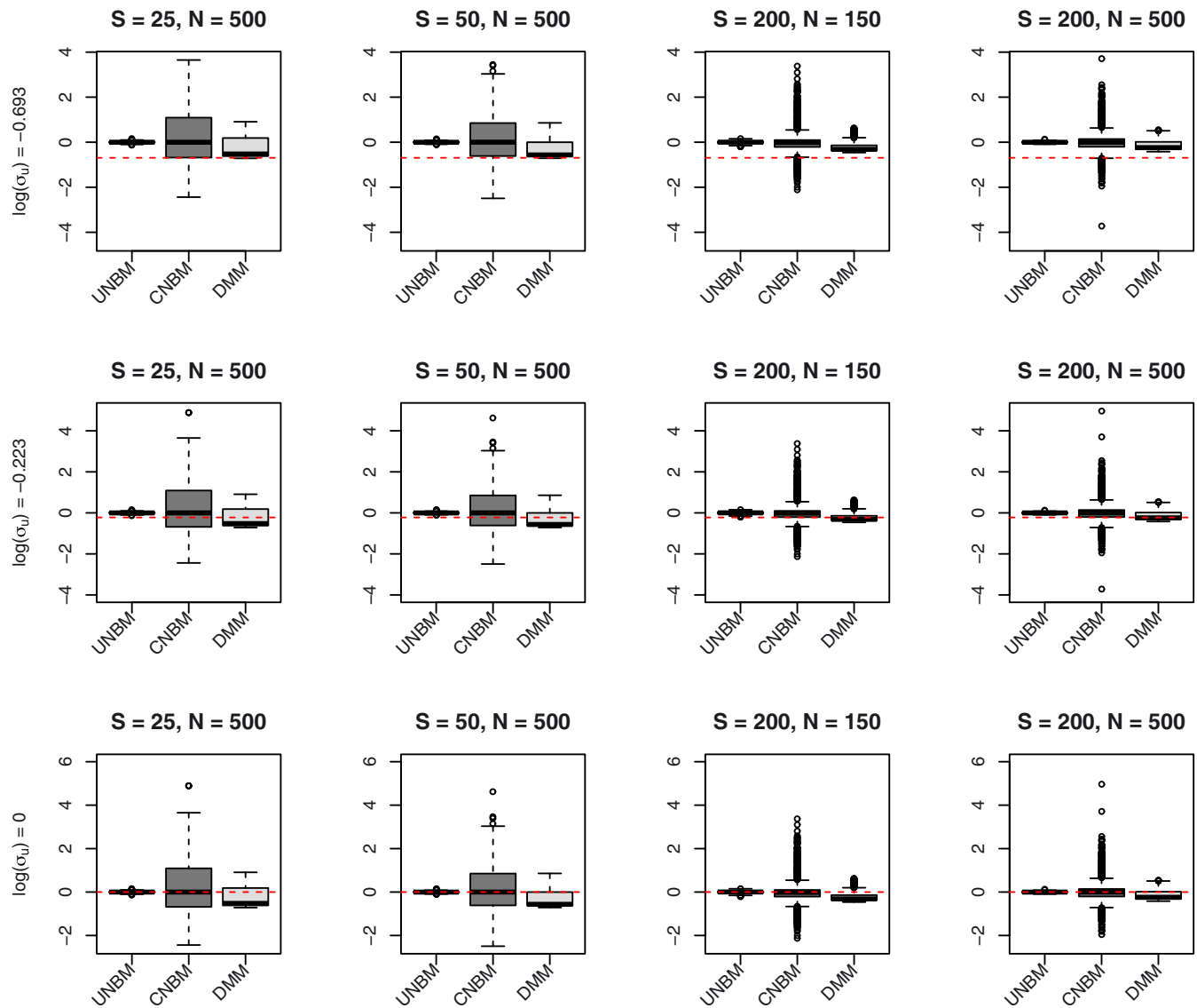
FIGURE 3 Estimates for the variance components obtained from three different models (UNBM, CNBM, and DMM) when data sets were generated using the UNBM model. CNBM, conditional negative-binomial mixed model; DMM, Dirichlet-multinomial mixed; UNBM, unconstrained negative binomial mixed [Colour figure can be viewed at wileyonlinelibrary.com ]
