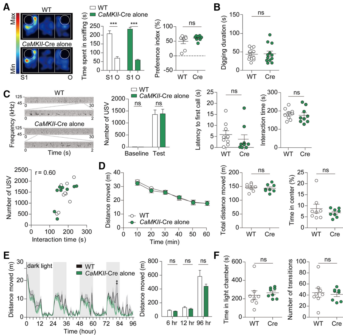
Figure 6. CaMKII-Cre mice show normal social interaction, digging, USVs, locomotor activity, and anxiety-like activity. A , Normal social interaction of CaMKII-Cre mice (10 weeks) in the three-chamber social interaction test, as shown by time spent sniffing a target (S1, O, or S2) and the social preference index. n = 8 mice for WT and CaMKII-Cre , *** p < 0.001 , ns (not significant), Student's t test. B , Normal digging in CaMKII-Cre mice (8 weeks), as shown by digging duration. n = 12 for WT and CaMKII-Cre , ns (not significant), Student's t test. C , Normal numbers of USVs (basal and female encounter) and latency to first call in CaMKII-Cre mice (9 weeks; males). Note that direct male–female social interaction is normal CaMKII-Cre mice, as measured by the time spent in sniffing, following, and mounting in males, which shows a positive correlation with the number of USVs ( r = 0.60 , n = 18 , WT and CaMKII-Cre combined, Pearson's correlation). n = 9 mice for WT and CaMKII-Cre , ns (not significant), Mann–Whitney U test (for latency to first call) and Student's t test. D , Normal locomotor activity of CaMKII-Cre mice (9 weeks) in the open-field test under 100 lux condition. Note that these mice also show normal anxiety-like behavior, as evidenced by the normal time spent in the center region of the open-field arena. n = 8 for WT and CaMKII-Cre , ns (not significant), two-way ANOVA, Student's t test, and Mann–Whitney U test (for time in center). E , Normal locomotor activity of CaMKII-Cre mice (11 weeks) in the LABORAS test, as shown by distance moved. n = 8 mice for WT and 7 for CaMKII-Cre , ** p < 0.01 , ns (not significant), two-way ANOVA, Student's t test (for 6 and 12 h), and Mann–Whitney U test (for 96 h). F , Normal anxiety-like behavior of CaMKII-Cre mice (10 weeks) in the light–dark test. n = 8 mice for WT and CaMKII-Cre , ns (not significant), Student's t test and Mann–Whitney U test (for time in light chamber).
