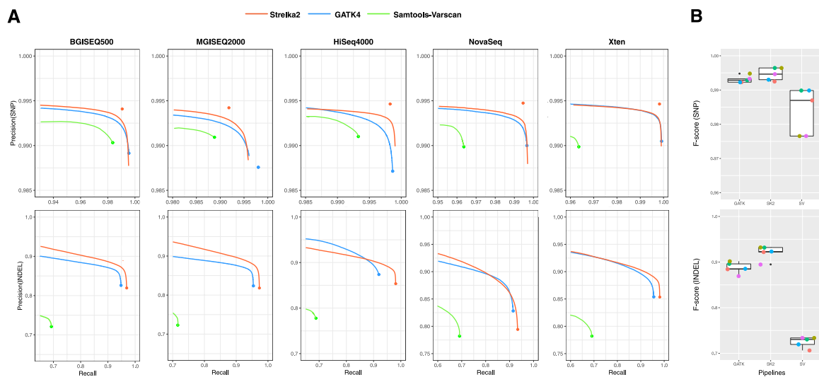
Figure 5. The summary of variants calling performances of multiple combinations in WGS datasets. (A) Accuracy of SNPs (up) and INDELS (down) calls for BGISEQ500, MGISEQ2000, HiSeq4000, NovaSeq and Xten WGS datasets. Large solid circles indicate the pass threshold of each combination. (B) Box plot indicates the distribution of F-score of multiple combinations in calling SNPs (up) and INDELS (down).
