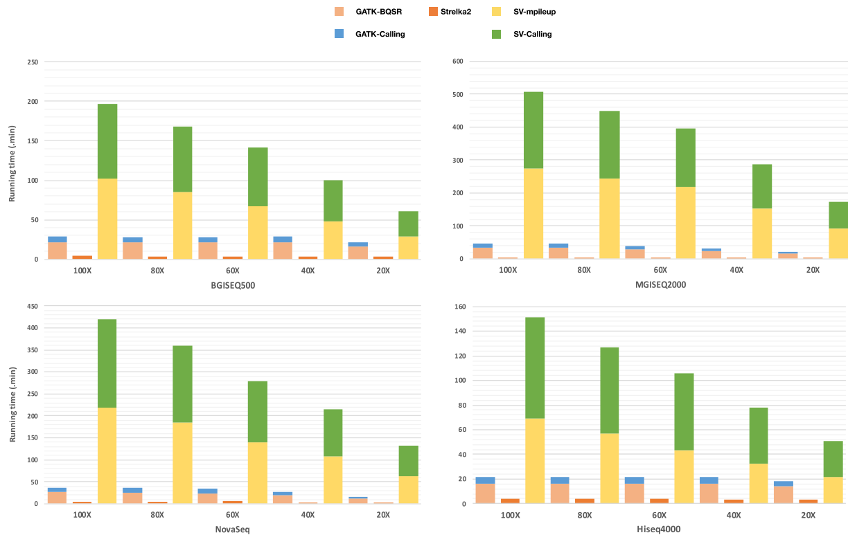
Figure 4. Variant calling runtime of multiple combinations in WES datasets. The variant calling runtime of each combination run on a Tianhe-2 supercomputer with 24 virtual CPUs and 88 GiB of memory. All combinations were configured to schedule tasks over all 24 virtual CPUs. The coverages of the down-sampled datasets were approximately 20X, 40X, 60X, 80X, 100X, respectively. Among them, variants calling in SK2 sets 24 threads, GATK used the default setting thread in BQSR and 24 threads setting in variants calling, and SV used the default setting thread in mpileup and variants calling.
