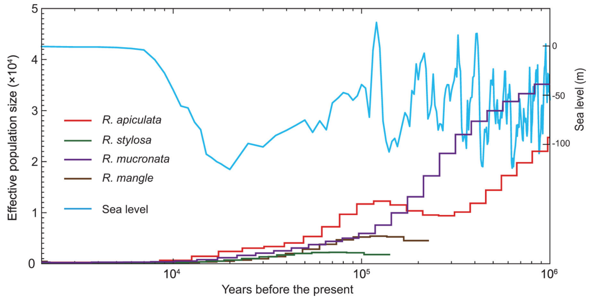
Figure 5. Rhizophora mangrove demography. Historical effective population size ( N_e , y-axis) changes going back in time (x-axis). The changes in N_e are inferred using the PSMC method [48], which relies on the varying level of genetic diversity in different DNA segments across the genome as a basis for the inference of historical N_e changes. In this graph, the generation time ( g ) is set to 20 years and the mutation rate ( \mu ) is 1.6 \times 10^{-8} /bp/generation. Historical sea-level fluctuations are plotted for comparison (blue line) [50].
