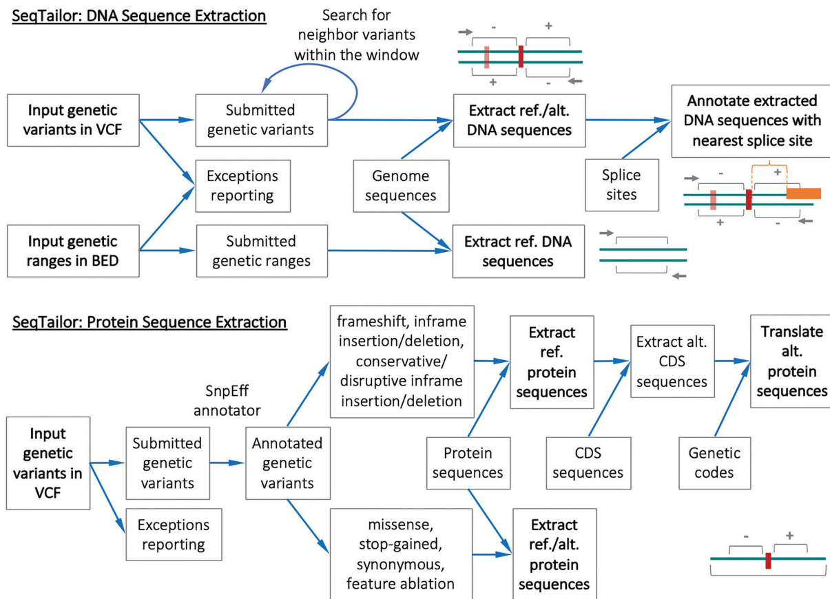
Figure 2. The framework of the SeqTailor webservice for DNA sequence extraction (upper) and protein sequence extraction (lower).
