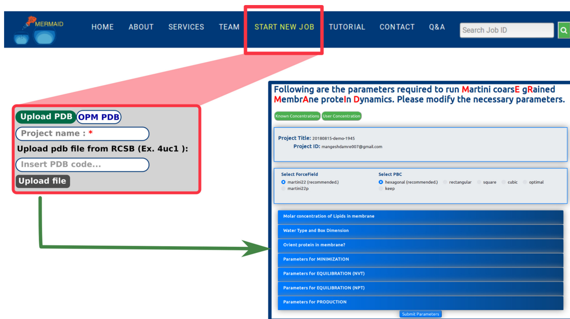
Figure 1. MERMAID web server interface (Start page, Parameter page): MERMAID provides two ways to submit a protein structure: a) from OPM database, or b) the user can upload the protein structure from a local system. After uploading the protein structure, MERMAID will redirect the user to parameter page.
