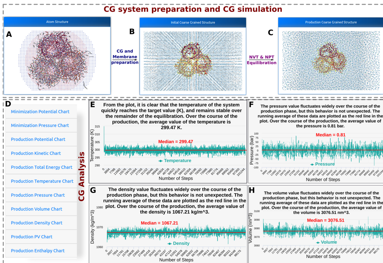
Figure 3. MERMAID server output. The upper panel shows the trimeric protein structure of the E. coli OmpF porin (PDB accession code: 3POX) in (A) atomistic description, (B) initial coarse-grained structure embedded in a coarse-grained membrane, (C) coarse-grained structure from the last frame of production run. A list of the analysis performed on the CG simulation (D). (E–H) shows the plots for temperature, pressure, system density, and system volume respectively.
