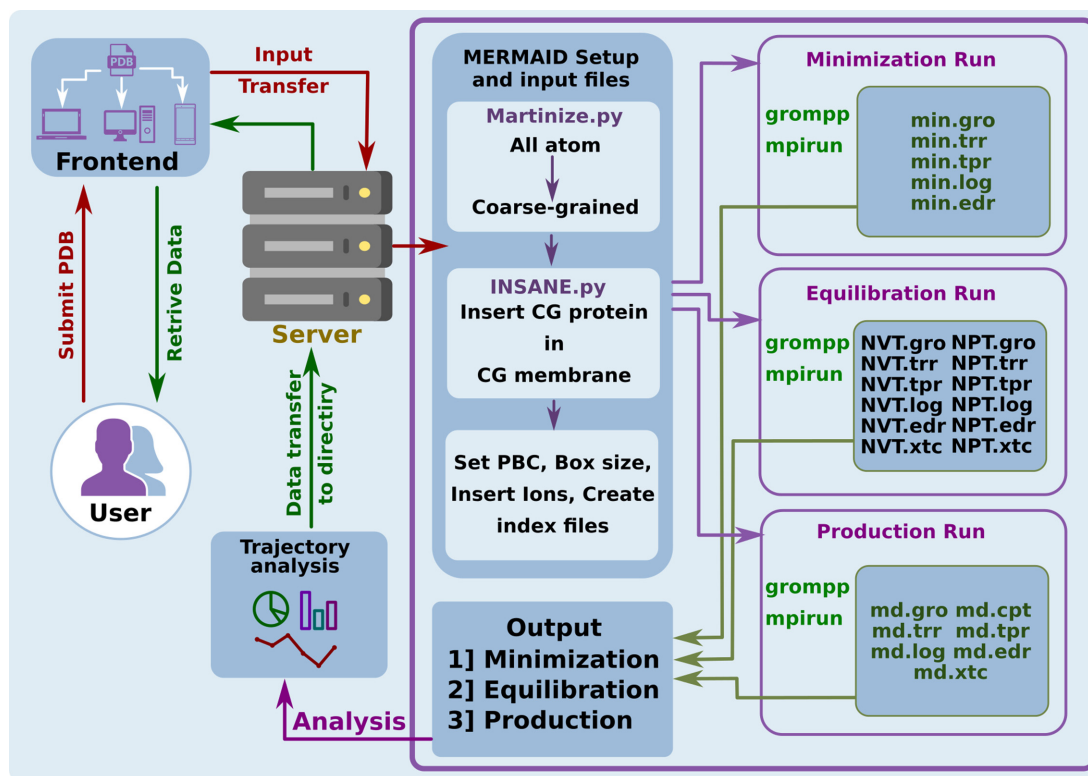
Figure 2. Workflow of the web server. The submitted protein structure is then converted into coarse-grained structure and inserted into CG membrane to form a complex structure. The structure then undergoes minimization, equilibration and production run respectively. Every phase of the coarse-grained simulation is analysed and can be visualised. Lastly, all the results can be downloaded from our server.
