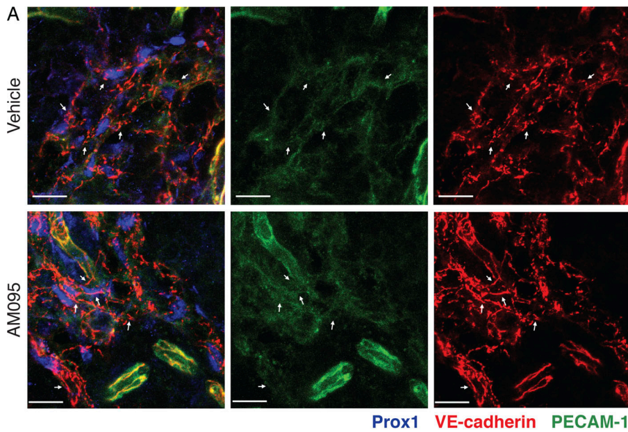
Figure 8. LPAR1 inhibits the formation of continuous junctions in LECs. (A) Lymph node sections (35 \mu\text{m} ) from vehicle or 8-h AM095-treated mice were stained with Prox1 (blue), VE-cadherin (red), and PECAM-1 (green). Arrows indicate VE-cadherin-positive adherens junctions. Bars, 10 \mu\text{m} . (B) Quantification of junctional length in the above confocal images. Confocal images ( n = 16 ) from three to five lymph nodes from two mice for each group were analyzed as described, and junctions of various lengths were quantified. Data are expressed as mean \pm SD. P values were determined using a two-way ANOVA followed by Sidak's multiple comparisons test comparing vehicle to AM095; **, P \leq 0.0021 ; ****, P \leq 0.0001 .
