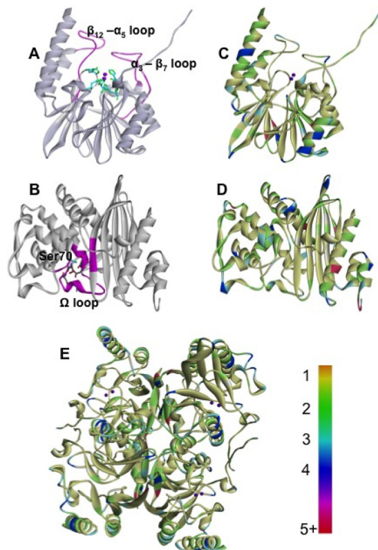
FIG 2 Protein structure and amino acid variability in the L1 and L2 \beta -lactamases. (A) Structure of L1 (PDB ID 2IOA ) displaying the Zn-binding residues as cyan sticks, Zn ions as purple spheres, and mobile loops in magenta. (B) Structure of L2 (PDB ID 1N4O ) displaying important catalytic residues in sticks with Ser70 highlighted in cyan and the \Omega -loop in magenta. (C and D) Amino acid variability in the L1 (C) and L2 (D) enzymes. Sequences obtained from 130 clinical strains and their reference sequences previously described by Avison et al. (21) were aligned, and variability per residue is indicated by the color scale shown at the bottom right from a conserved position (yellow) to a position where two (green), three (cyan), four (blue), or five or more (magenta) different amino acids can be found. (E) Mapping of amino acid variability in the crystal structure of the L1 tetramer (PDB ID 2QIN ).
