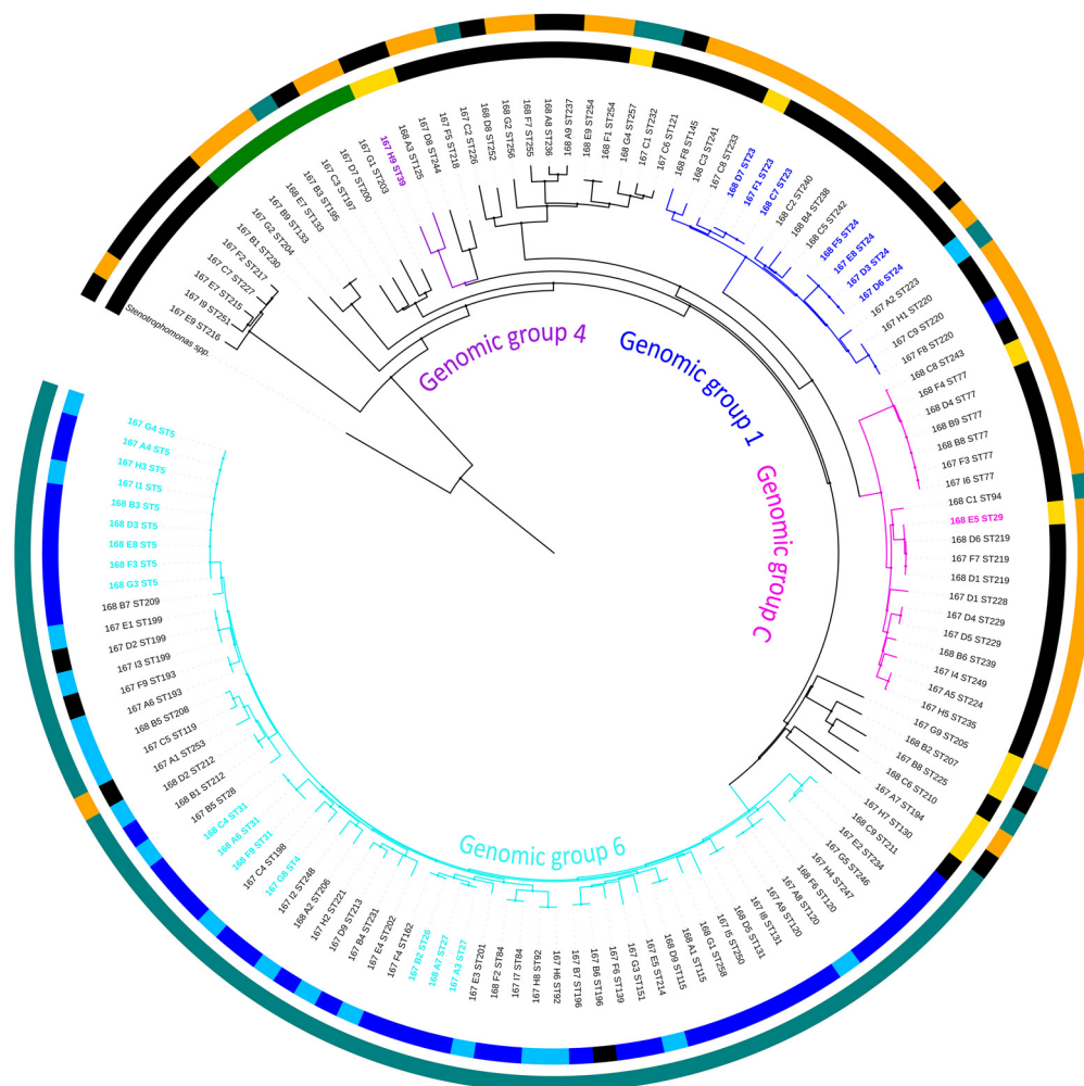
FIG 7 Putative association of specific types of L1 and L2 -lactamases with genomic group 6. Phylogenetic analysis of S. maltophilia from concatenated sequences of the seven housekeeping gene fragments (3,591 nt). A consensus UPGMA tree shows the structure of the studied S. maltophilia population ( n = 130 ). Branch length represents the genetic distance, with the scale bar indicating the number of substitutions per nucleotide position. The tree was rooted with a sequence from Stenotrophomonas spp. (not S. maltophilia ). The genomic group designation according to MLST in the original study by Kaiser et al. (20) is indicated by colored branches: cyan, genomic group 6; blue, genomic group 1; purple, genomic group 4; magenta, genomic group C. Known STs belonging to each genomic group are highlighted in their corresponding color. Internal and external rings indicate L1 and L2 types, respectively.
