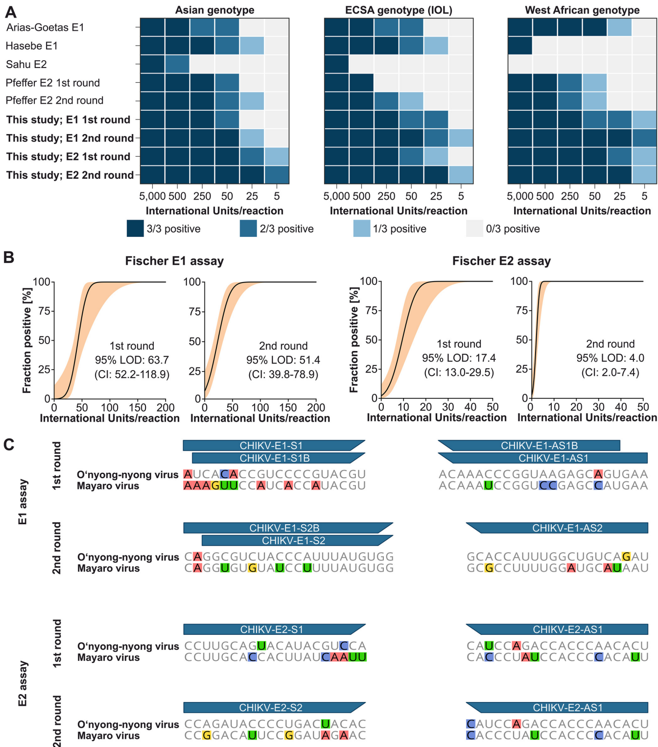
FIG 2 Assay validation. (A) Determination of robustness across CHIKV genotypes. New assays (boldface) and reference assays were tested with CHIKV RNA of the Asian, ECSA, and West African genotypes. (B) Determination of lower limits of detection (LOD) for the new PCR assays. Quantified RNA of the Asian CHIKV genotype was diluted stepwise and was tested in eight replicates with first-round assays. Probit analyses were done using R 3.5.2. (C) Conservation of primer target regions among representative Mayaro (NC003417) and O'nyong-nyong (NC001512) viruses. Mismatches with the new CHIKV assays are highlighted.
