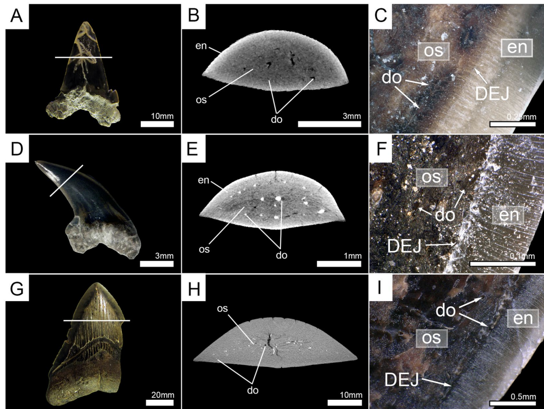
Figure 5. Horizontal virtual micro-CT sections and manual tooth sections of extinct lamniform sharks. (A–C) † Dwardius woodwardi (Lamniformes incertae fam.) (EMRG-Chond-T-53); (D–F) † Squalicorax sp. (†Anacoracidae) (EMRG-Chond-T-54); (G–I) † Otodus megalodon (†Otodontidae) (EMRG-Chond-T-57). White lines indicate the plane of the sections. do, dentinal osteons; en, enameloid; os, osteodentine.
