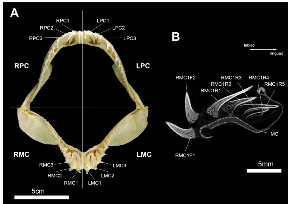
Figure 8. Terminology used to describe the topology of teeth within the jaws and tooth files. (A) Jaws of Pseudocarcharias kamoharai (Inv.nr. 7-693/RZ) in frontal view, (B) virtual section through the tooth file RMC1. F, functional tooth; F1, first (oldest) functional tooth; F2, second functional tooth; LMC, left Meckel's cartilage; LPC, left palatoquadrate cartilage; MC, Meckel's cartilage (lower jaw); PQ, palatoquadrate cartilage (upper jaw); R, replacement tooth; R1, first (oldest) replacement tooth; R2, second replacement tooth; R3, third replacement tooth; R4, fourth replacement tooth; R5, fifth replacement tooth; RMC, right Meckel's cartilage; RPC, right palatoquadrate cartilage.
