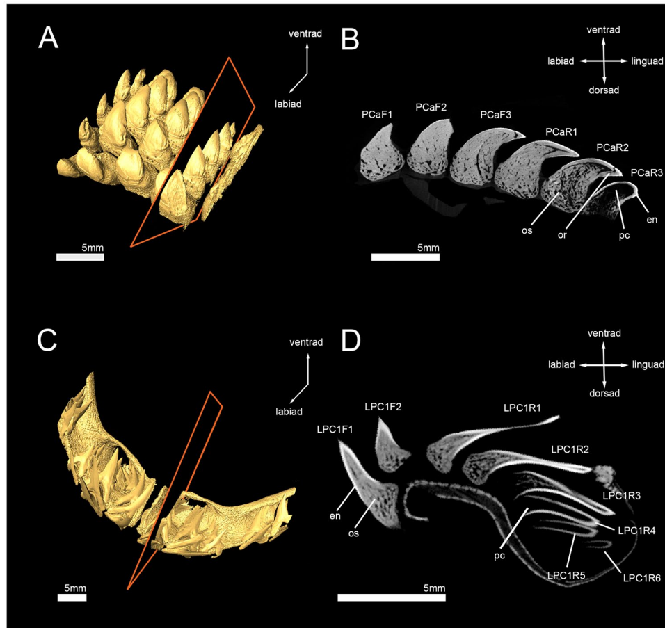
Figure 1. 3D micro-CT isosurfaces of the upper jaws and 2-D images of the virtually sectioned tooth row reveal two different patterns of tooth mineralization in lamniform sharks. The basking shark Cetorhinus maximus (7-692/RZ) ( A,B ) develops two layers of dentine (orthodentine and osteodentine representing the pseudoosteodont histotype), while the crocodile shark Pseudocarcharias kamoharai (7-693/RZ) ( C,D ) lacks orthodentine and only develops osteodentine (osteodont histotype). en, enameloid; or, orthodentine; os, osteodentine; pc, pulp cavity.
