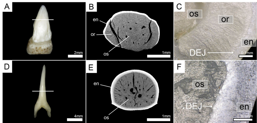
Figure 2. Horizontal virtual micro-CT sections and manual tooth sections of the basking shark ( Cetorhinus maximus , Cetorhinidae) (EMRG-Chond-T-24) and the crocodile shark ( Pseudocarcharias kamoharai , Pseudocarchariidae) (EMRG-Chond-T-28). (A) picture of a functional tooth prior to the tooth section, (B) virtual section, and (C) tooth section of C. maximus under normal light illustrating the presence of two layers of dentine - compact orthodontine surrounding a core of osteodentine. (D) picture of a functional tooth prior to the tooth section, (E) virtual section, and (F) tooth section of P. kamoharai under polarized light illustrating the presence of one layer of dentine - osteodentine. White lines indicate the approximate plane of the sections. do, dentinal osteons; en, enameloid; or, orthodontine; os, osteodentine.
