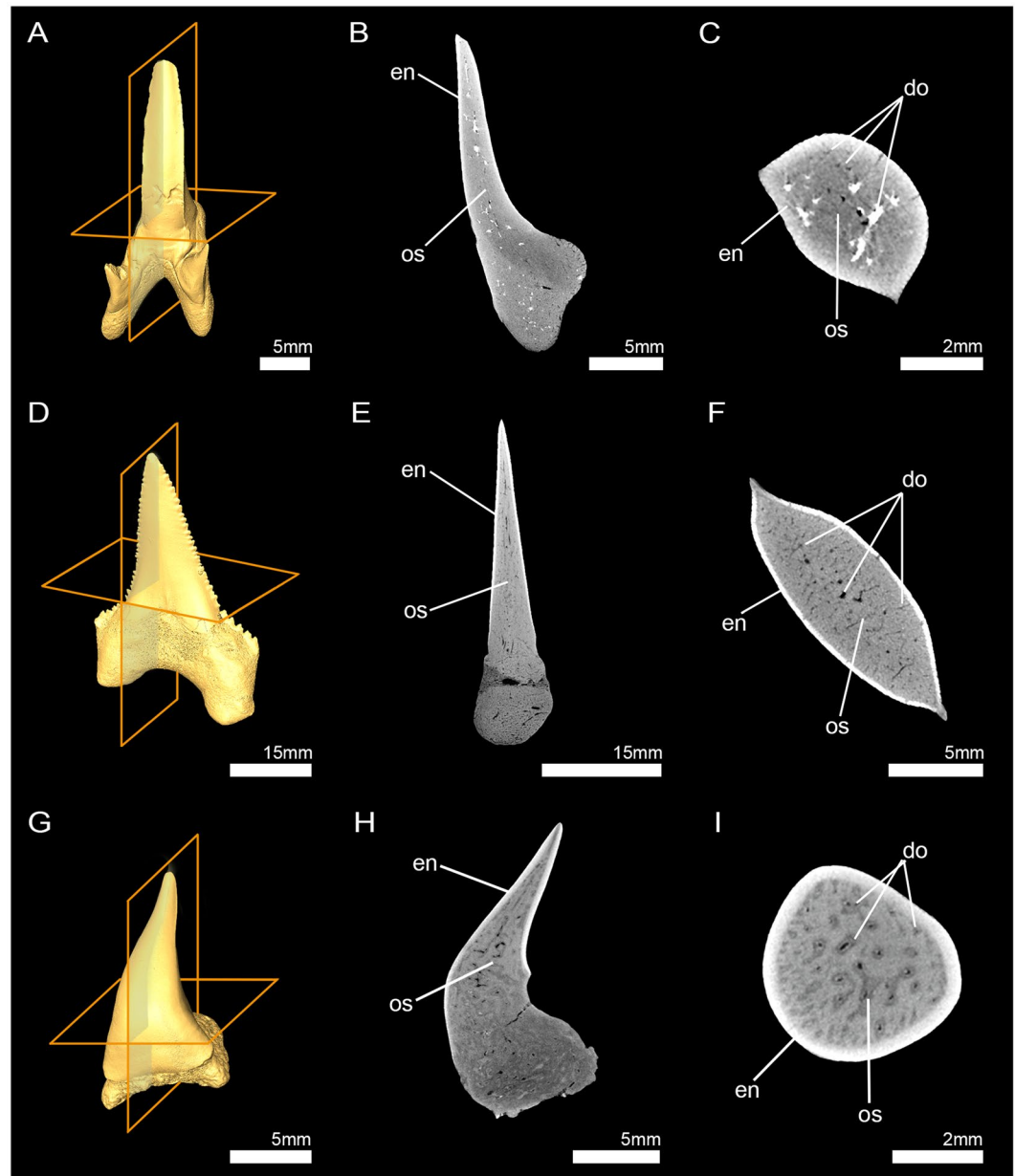
Figure 4. 3D reconstructions and virtual micro-CT sections (sagittal and axial plane) of fossil lamniform shark teeth. (A–C) † Leptostyrax sp. (†Eoptolamnidae (sensu Kriwet et al. 35 ) (Inv.nr. 7–690); (D–F) † Palaeocarcharodon orientalis (Lamniformes incertae fam.) (EMRG-Chond-T-50); (G–I) Megachasma pelagios (Megachasmidae) (EMRG-Chond-T-44). do, dental osteons; en, enameloid; os, osteodentine.
