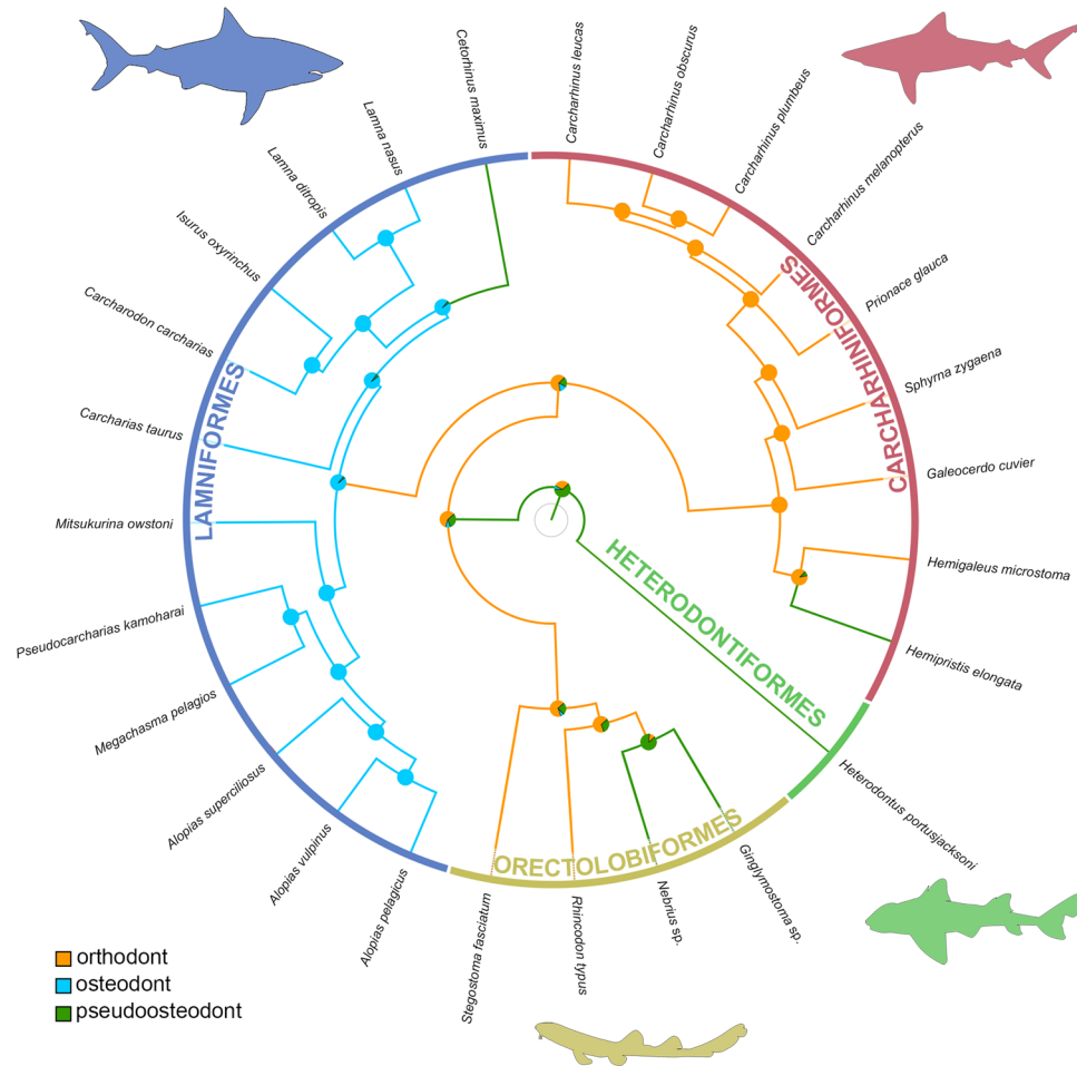
Figure 7. Stochastic character mapping of tooth histotypes and ancestral state reconstructions in sharks of the superorder Galeomorpha. The maximum credibility tree of the galeomorph sharks is based on whole mtDNA sequences. Ancestral states at the nodes are coded as pie charts proportions of the probability distribution, calculated from 100 stochastic mappings for the three histotypes present (orthodonty, osteodonty and pseudoosteodonty).
