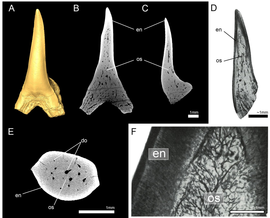
Figure 6. High resolution micro-CT images of virtual tooth sections and manual tooth sections of the original description of † Palaeocarcharias stromeri . (A) 3D reconstruction, (B,C,E) virtual tooth sections in (B) frontal, (C) sagittal and (E) axial view. (D,F) are modified pictures of the manual tooth sections from the original description of † P. stromeri by Beaumont 10 . Do, dentinal osteons; en, enameloid; os, osteodentine.
