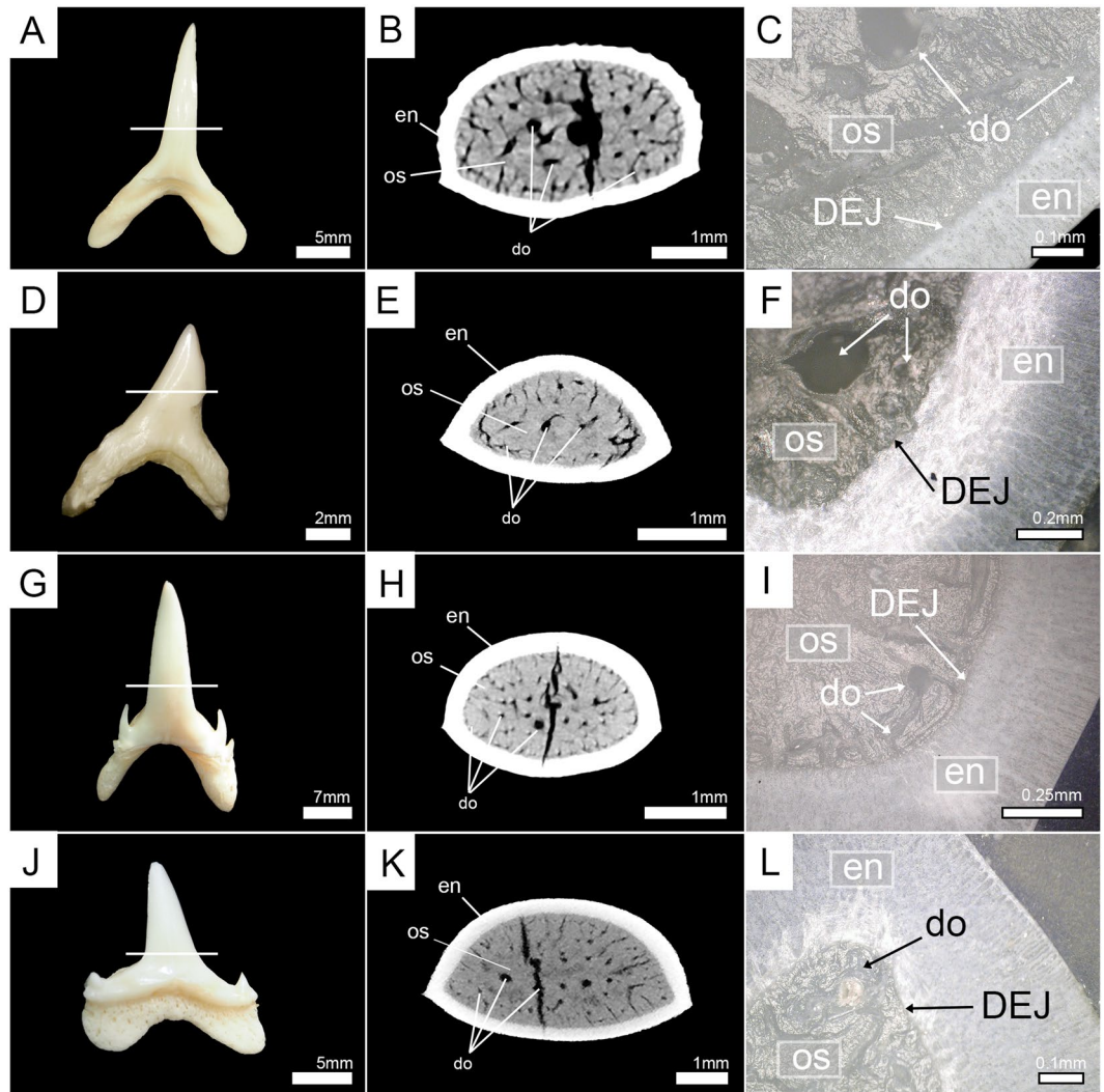
Figure 3. Horizontal virtual micro-CT sections and manual tooth sections of extant lamniform sharks under normal light. (A–C) goblin shark ( Mitsukurina owstoni , Mitsukurinidae) (EMRG-Chond-T-1); (D–F) common thresher ( Alopias vulpinus , Alopiidae) (EMRG-Chond-T-27); (G–I) smalltooth sand tiger ( Odontaspis ferox , Odontaspidae) (EMRG-Chond-T-2); (J–L) porbeagle shark ( Lamna nasus , Lamnidae) (EMRG-Chond-T-4). White lines indicate the approximate plane of the sections. do, dentinal osteons; en, enameloid; os, osteodentine.
