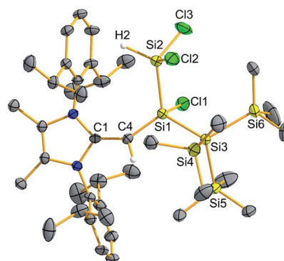
Fig. 4 Molecular structure of (\text{M}^e\text{IPrCH})\text{SiCl}(\text{SiHCl}_2)\{\text{Si}(\text{SiMe}_3)_3\} ( 5 ) with thermal ellipsoids plotted at a 30% probability level. All hydrogen atoms (except the vinylic hydrogen and silane hydrogen) were omitted for clarity. Selected bond lengths [Å] and angles [°]: C1–C4 1.394(7), C4–Si1 1.789(5), Si1–Si2 2.364(2), Si1–Cl1 2.170(2), Si2–H2 1.50(7), Si2–Cl2 2.076(3), 2.074(3), Si1–Si3 2.358(2); Si2–Si1–Si3 109.81(9), Si2–Si1–Cl1 100.27(9), Si2–Si1–C4 118.15(19).
