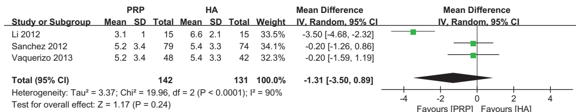
Figure 5. Forest plot and meta-analysis of Lequesne index scores.
