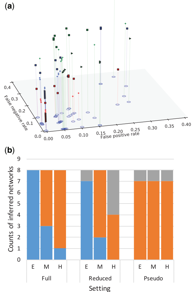
Fig. 4. Accuracy of the inferred networks, and comparison to maximum pseudo-likelihood. (a) The false positives and false negatives for the datasets where the inferred network is not identical to the true network. Squares correspond to hard networks, crosses correspond to medium-difficulty networks and triangles correspond to easy networks. Blue, red and green correspond to results based on the full and reduced sets of trinetts, and maximum pseudo-likelihood, respectively. (b) The accuracy of our method on the full set of trinetts (left set of bars) and on the reduced set of trinetts (middle set of bars), and the accuracy of maximum pseudo-likelihood (right set of bars). Blue corresponds to the datasets where the inferred network is identical to the true network; orange corresponds to the datasets where the inferred network contains a backbone network that is present in the true network; grey corresponds to all other cases
