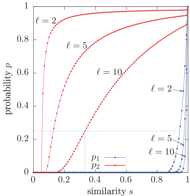
Fig. 3. The relationships between the similarity thresholds s_1 and s_2 , and the probabilities p_1 and p_2 , for n = 100, k = 5 . Given a probability, e.g. p_1 = p_2 = 0.25 shown by the horizontal gray line, the OMH method can distinguish between similarities below s_2 (below left vertical gray line) and from similarities above s_1 (above the right vertical gray line). The functions are defined at discrete points, when ns is integral, represented by the circles and squares
