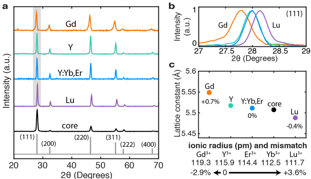
Figure 2: Structural characterization and induced strain
