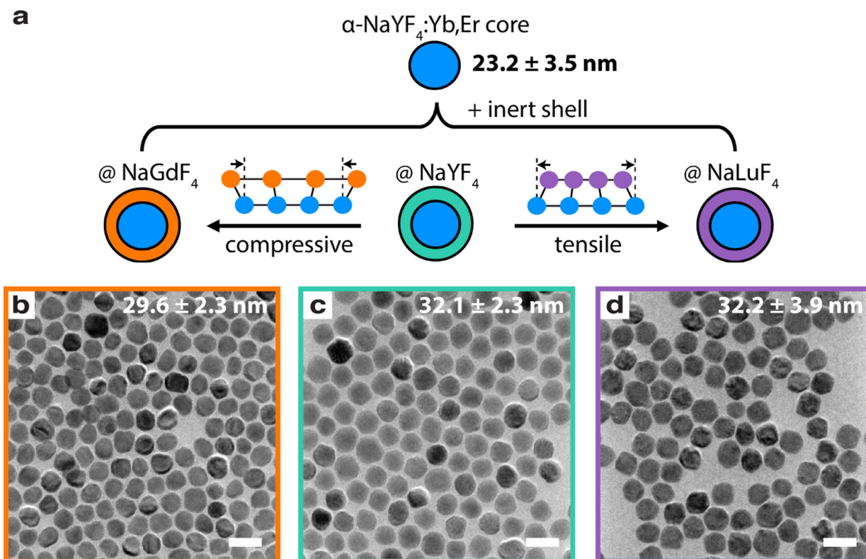
Figure 1: Schematic and micrographs of core-shell nanoparticles
