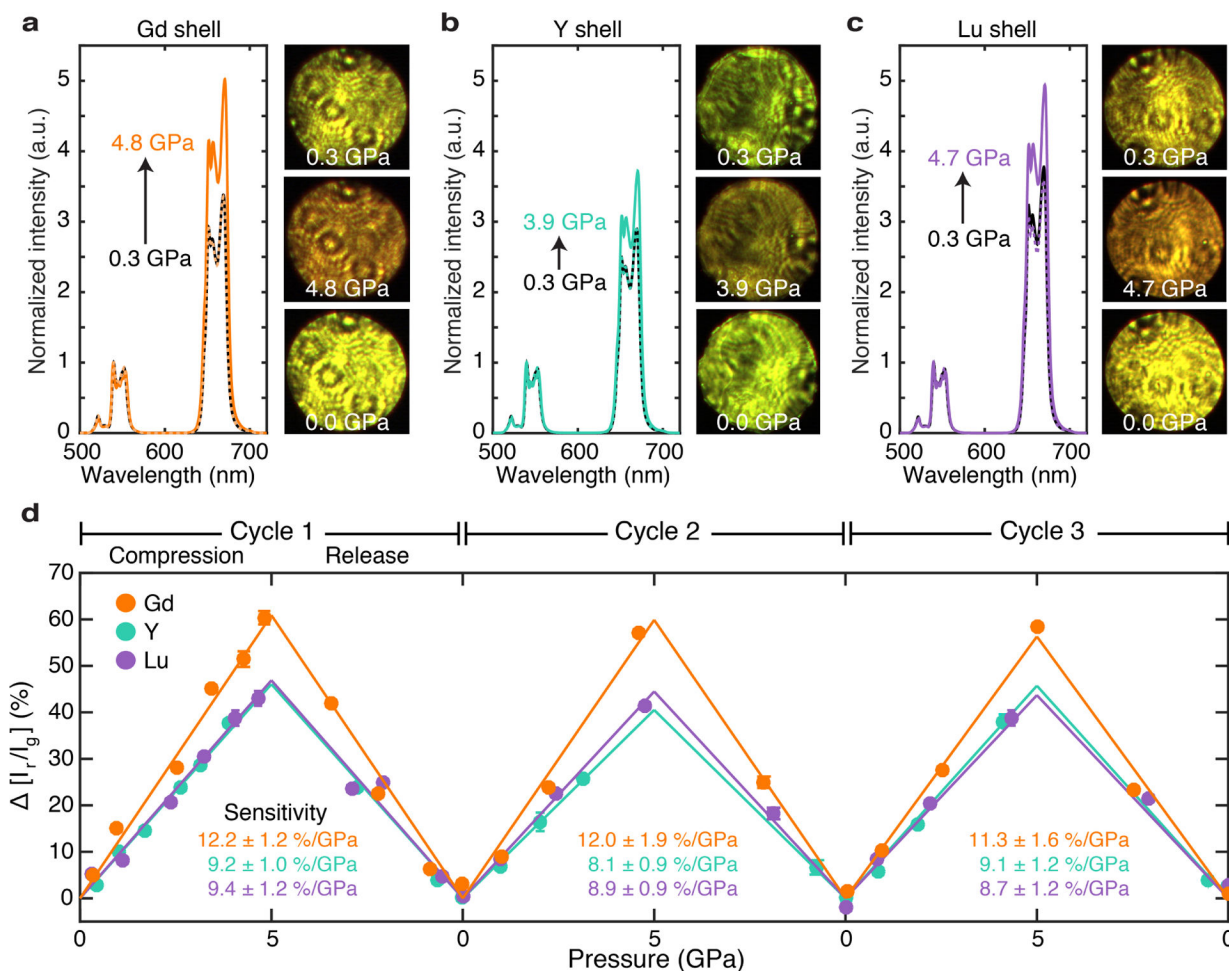
Figure 4: Mechanosensitivity or color response of core-shell UCNPs
