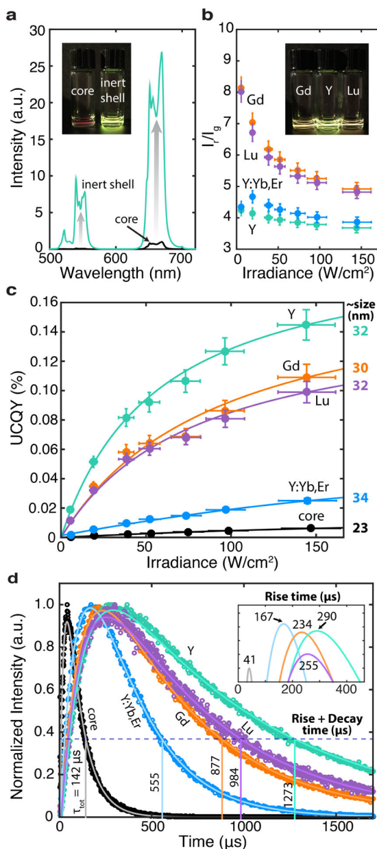
Figure 3: Upconversion emission properties
