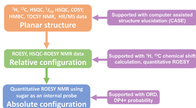
Figure 1. Overview of the systematic structure determination workflow.
