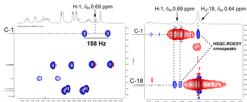
Figure 4. Left: J -coupled HSQC showing a large ^1J_{\text{CH}} of 158 Hz, characteristic of a cyclopropane. Right: HSQC-ROESY cross-peak suggesting cis-fusion of rings A, B for 1 .
