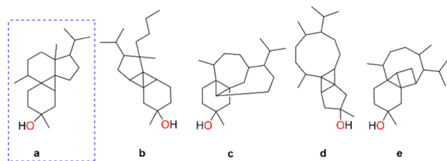
Figure 5. Top five structural hits for the diterpene core of 1 generated by MestReNova CASE. The structure a in the hatched box represents the top hit.
