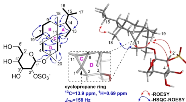
Figure 3. Left: Key COSY (bold lines), HMBC (blue arrows), Right: HSQC-ROESY (blue arrow), and ROESY (red arrows) correlations for 1 .
