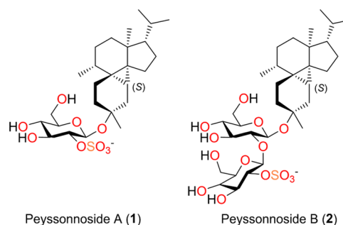
Figure 2. Novel diterpene glycosides peyssonosides A–B (1–2) from the marine red alga Peyssonnelia sp.
