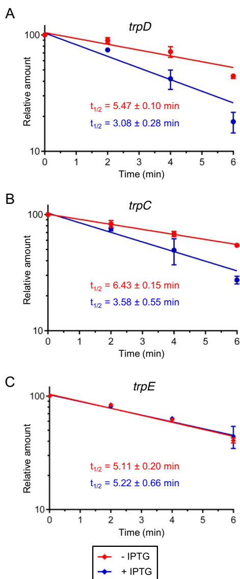
Figure 5. The sRNA rnTrpL destabilizes the polycistronic trpDC mRNA. At an OD_{600nm} of 0.5, one half of a liquid culture of strain 2011 \Delta trpL (pSRKTe-rnTrpL) was supplemented with IPTG for 10 min to induce lacZ'-rnTrpL production, while the other half was incubated without IPTG. Then, rifampicin was added to both cultures and RNA was isolated at time points 0, 2, 4 and 6 min after rifampicin addition. Relative mRNA levels in induced (blue) and uninduced cultures (red) were determined by qRT-PCR analysis and half-lives ( t_{1/2} , in min) were calculated from three independent experiments, each with two technical replicates. The analysis was performed with primers specific for trpD (A), trpC (B) and trpE (C). The analysis with ppiD -, moaC - and moeA -specific primers is shown in Supplementary Figure S4.
