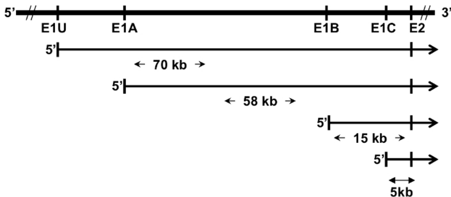
Figure 1. Diagram of the genomic alignment of ESTs with sequence identity to Bcrp1 exon 2 with murine chromosome 6. These alignments were identified in a dbEST BLAST search performed in April, 2015. Four distinct alignments were found, corresponding to Bcrp1 alternative first exons E1U, E1A, E1B, and E1C. This figure is reproduced from a previous publication 5 . Please click here to view a larger version of this figure.
