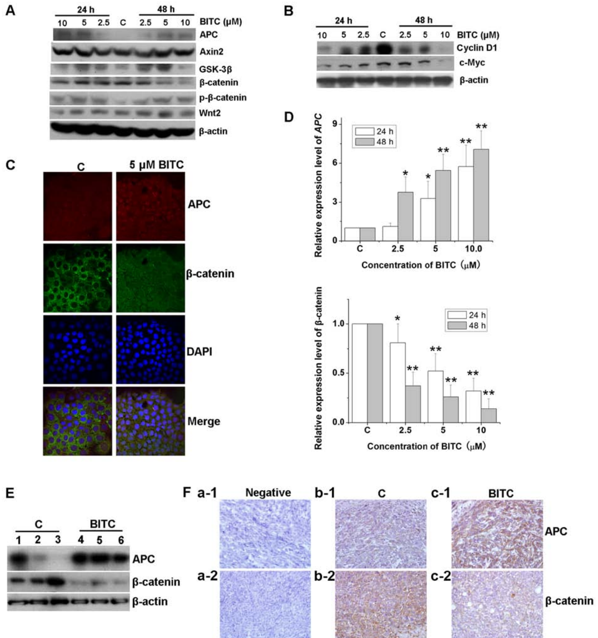
Figure 4. BITC regulates the Wnt/ \beta -catenin pathway and the APC/ \beta -catenin complex. 4T1-Luc cells were treated with various concentrations of BITC as indicated for 24 and 48 h. Total protein lysates were immunoblotted for (A) APC, Axin2, GSK-3 \beta , \beta -catenin, p- \beta -catenin and Wnt2, and (B) cyclin D1 and c-Myc protein expression. \beta -actin was used as the internal control. (C) Immunofluorescence assay was performed to evaluate the expression and subcellular location of APC and \beta -catenin protein (magnification, x1,000). (D) 4T1-Luc cells were treated with various concentrations of BITC as indicated for 24 and 48 h, and total RNA was isolated and reverse transcribed. The mRNA expression levels of APC and \beta -catenin were detected via reverse transcription-quantitative PCR analysis. * P < 0.05 , ** P < 0.01 vs. C. (E) Protein lysates isolated from the tumors of control or BITC-treated mice were subjected to western blot analysis for APC and \beta -catenin. 1-6 indicated different mice. (F) Tumors from control and BITC-treated mice were subjected to immunohistochemical analysis using APC and \beta -catenin antibodies (magnification, x400). APC, adenomatous polyposis coli; BITC, benzyl isothiocyanate; C, control; DAPI, 4',6'-diamidino-2-phenylindole; GSK-3 \beta , glycogen synthase kinase-3 \beta .
