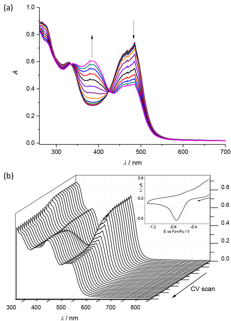
Figure 7. In situ UV-vis-NIR spectroelectrochemistry for 1 in DMSO/ n\text{Bu}_4\text{NPF}_6 (scan rate of 10\text{ mV s}^{-1} , Pt-microstructured honeycomb working electrode): (a) evolution of UV-vis spectra in 2D projection in forward scan in the region of the first reduction peak; (b) UV-vis spectra detected simultaneously upon the cyclic voltammetric scan in 3D projection (Inset: the corresponding cyclic voltammogram).
