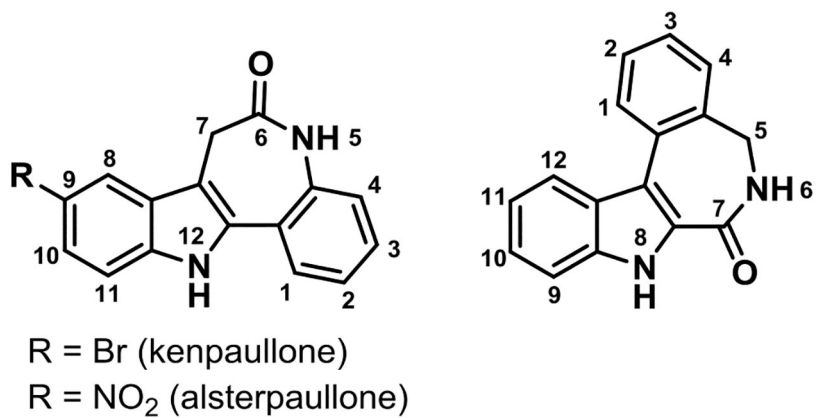
Chart 1. The indolo[3,2- d ]benzazepinone (pauillone) (left), vs the indolo[2,3- d ]benzazepinone backbone (right) with numbering schemes.
