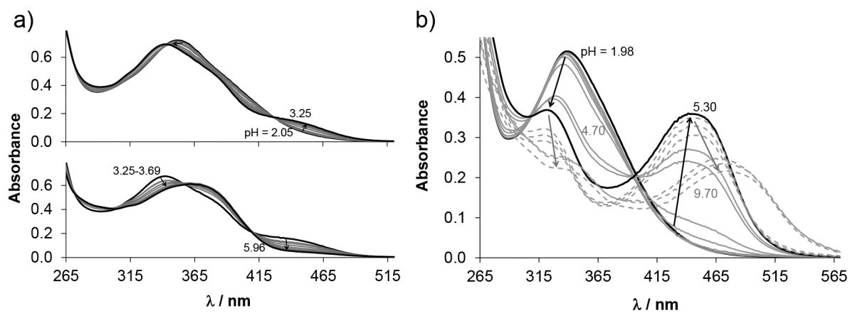
Figure 4. UV-vis spectra recorded for a) \text{HL}^3 and b) complex 3 at various pH values in 30–70% (w/w) DMSO-water solvent mixture. { c_{\text{ligand}} = c_{\text{complex}} = 12.5 \mu\text{M} ; T = 298 \text{ K} ; I = 0.10 \text{ M} (KCl); l = 2 \text{ cm} }.
