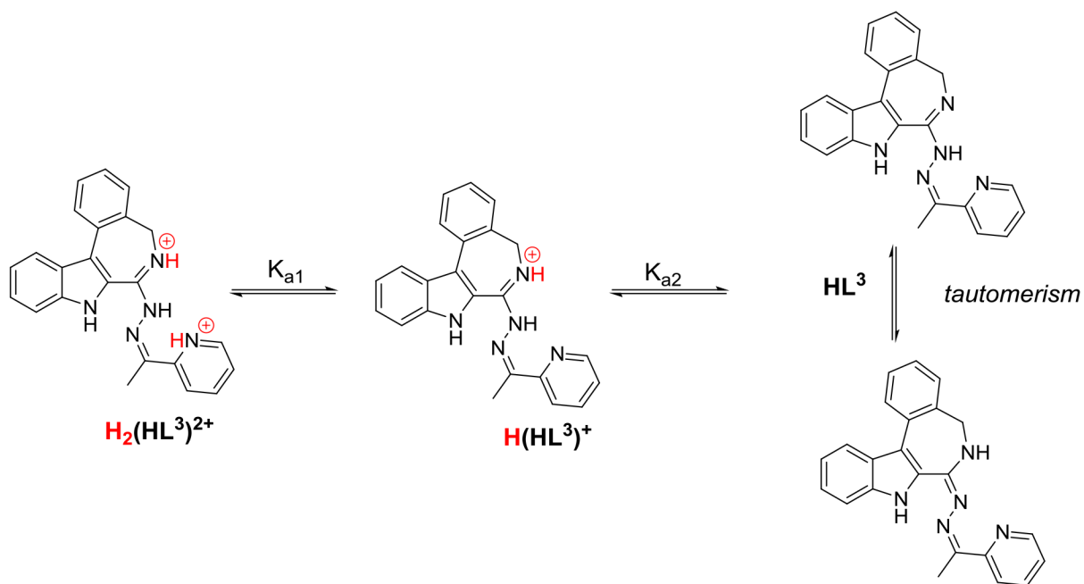
Chart 4. Stepwise deprotonation processes of the fully protonated form of \mathbf{HL}^3 and its tautomeric forms.
