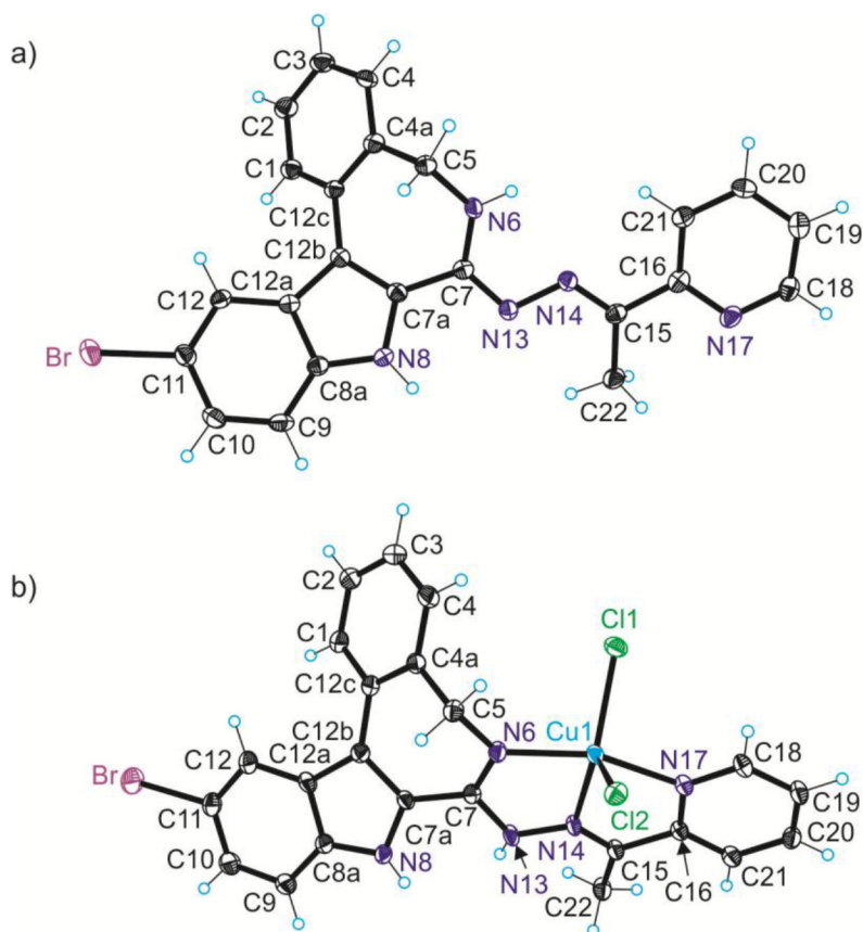
Figure 3. ORTEP views of a) proligand HL 4 and b) of [CuCl 2 ( HL 4 )] in 4 (co-crystallised solvent is omitted). Selected bond distances (Å) and bond angles (deg) in HL 4 : C5–N6 1.459(4), N6–C7 1.344(4), C7–N13 1.325(4), N13–N14 1.391(3), N14–C15 1.300(4); in 4 : Cu1–N6 2.011(2), Cu1–N14 1.986(2), Cu1–N17 2.057(3), Cu1–Cl1 2.2612(8), Cu1–Cl2 2.4327(9), C5–N6 1.470(4), N6–C7 1.295(4), C7–N13 1.376(4), N13–N14 1.366(3), N14–C15 1.285(4), N6–Cu–N14 78.83(10), N14–Cu–N17 77.34(10), Cu2–N28 2.010(2), Cu2–N36 1.968(2), Cu2–N39 2.035(3), Cu2–Cl3 2.2204(8), Cu2–Cl4 2.5321(9), N28–Cu2–N36 79.40(10), N36–Cu2–N39 78.40(10). Details of coordination geometry in 4 : \tau_5 (Cu1) = 0.28, \tau_5 (Cu2) = 0.28 (second crystallographically independent molecule).
