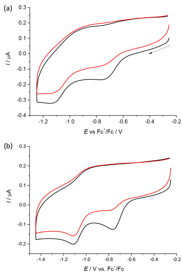
Figure 6. Cyclic voltammograms of (a) 1 and (b) 4 in DMSO/ n\text{Bu}_4\text{NPF}_6 at scan rate of 100 \text{ mV s}^{-1} at GC working electrode (black traces represent the first scan, while red traces the second scan).
