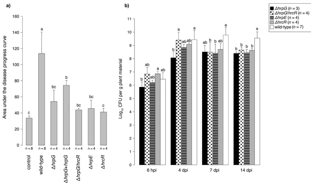
Fig. 3 (a) Mean areas under the disease progress curve (AUDPCs) from four replications for Lolium multiflorum genotype LmK-01 infected with Xanthomonas translucens pv. graminis strain 29 (Xtg29) deficient in genes encoding the type III secretion system (T3SS) compared with the wild-type strain. Means with different letters are significantly different ( P < 0.05 ) on the basis of a two-sided t -test using the Holm P value adjustment. The negative control treatment consisted of cutting the plants with scissors dipped in sterile physiological sodium chloride solution. (b) Colonization of L. multiflorum by Xtg29 and the Xtg29 strains deficient in T3SS genes. Bacterial population densities were determined for leaves of three or four different plants of LmK-01 sampled at 6 h post-infection (hpi) and 4, 7 and 14 days post-infection (dpi), counting the colony-forming units (CFU) of serial dilutions. For each time point, mean population densities and standard deviations were calculated. Means indicated with different letters are significantly ( P < 0.05 ) different on the basis of a two-sided t -test using the Holm P value adjustment.
