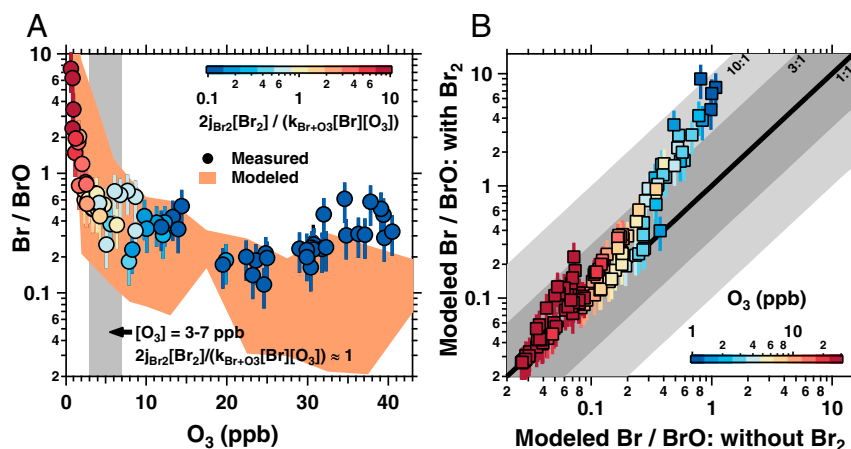
Fig. 3. (A) Measured Br/BrO ratios ( \text{ppt ppt}^{-1} ) as a function of measured \text{O}_3 . Data points are color-coded by 2j_{\text{Br}_2}[\text{Br}_2]/(k_{\text{Br}+\text{O}_3}[\text{Br}][\text{O}_3]) , calculated from measured \text{Br}_2 , Br, and \text{O}_3 ; the gray shading shows the \text{O}_3 levels for which this calculated ratio is \sim 1 . Orange shading shows the range in modeled Br/BrO ratios (Methods). (B) Modeled Br/BrO ratios, with/without constraining \text{Br}_2 , color-coded by measured \text{O}_3 . Shaded areas correspond to differences of factors of 3 and 10. Error bars represent propagated \text{Br}_2 measurement uncertainty; data below the limit of quantitation are excluded.
