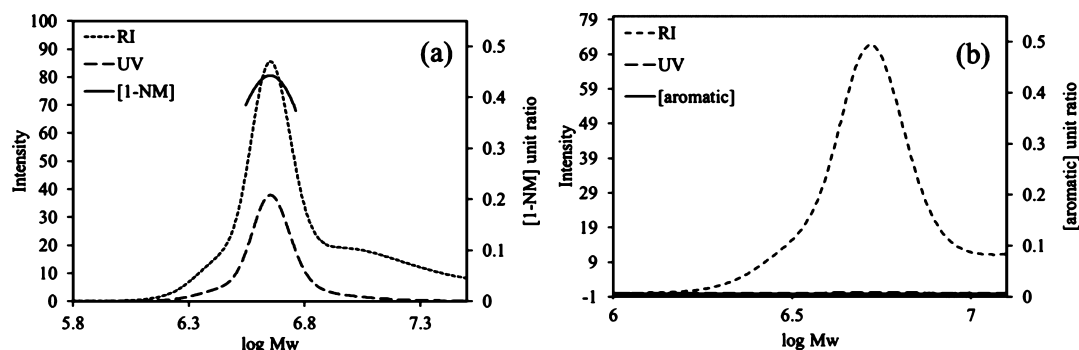
Figure 1. SEC profiles monitored by RI and UV detectors and (a) [1-NM] unit ratio for PCL (with 1-NM); (b) [aromatic] unit ratio for PCL (with butanol).
